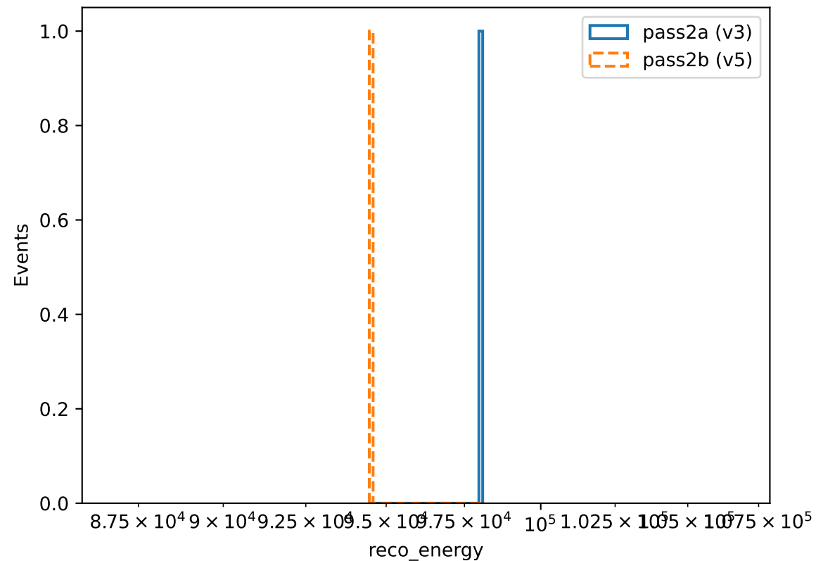
Distributions
