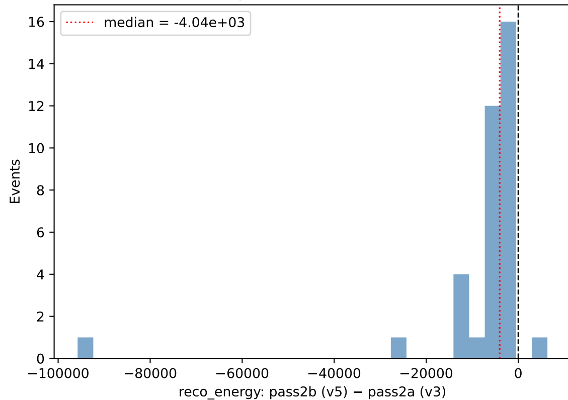
Event-by-event difference (N=36)
