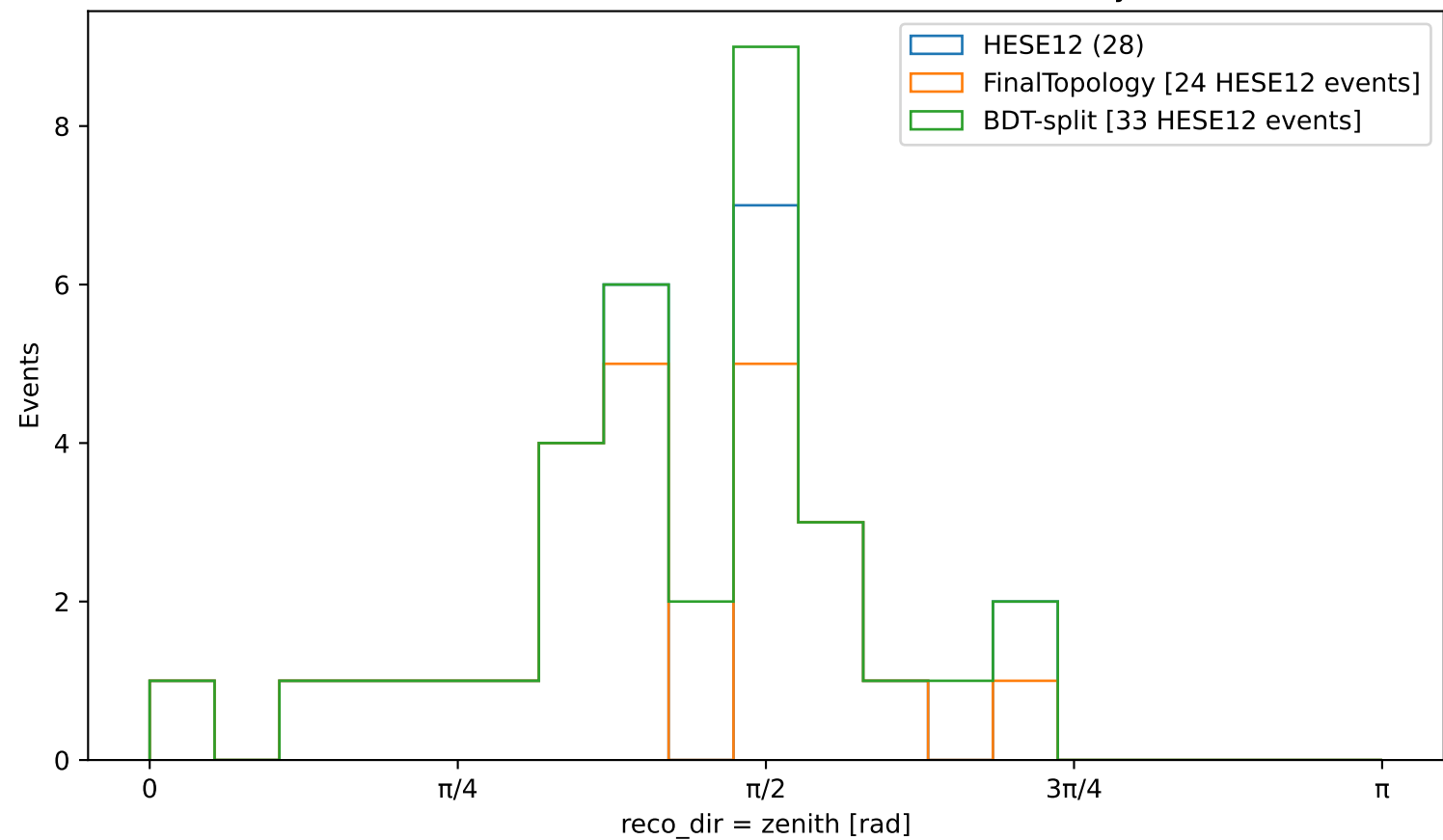
Track zenith distribution — HESE12 events only
