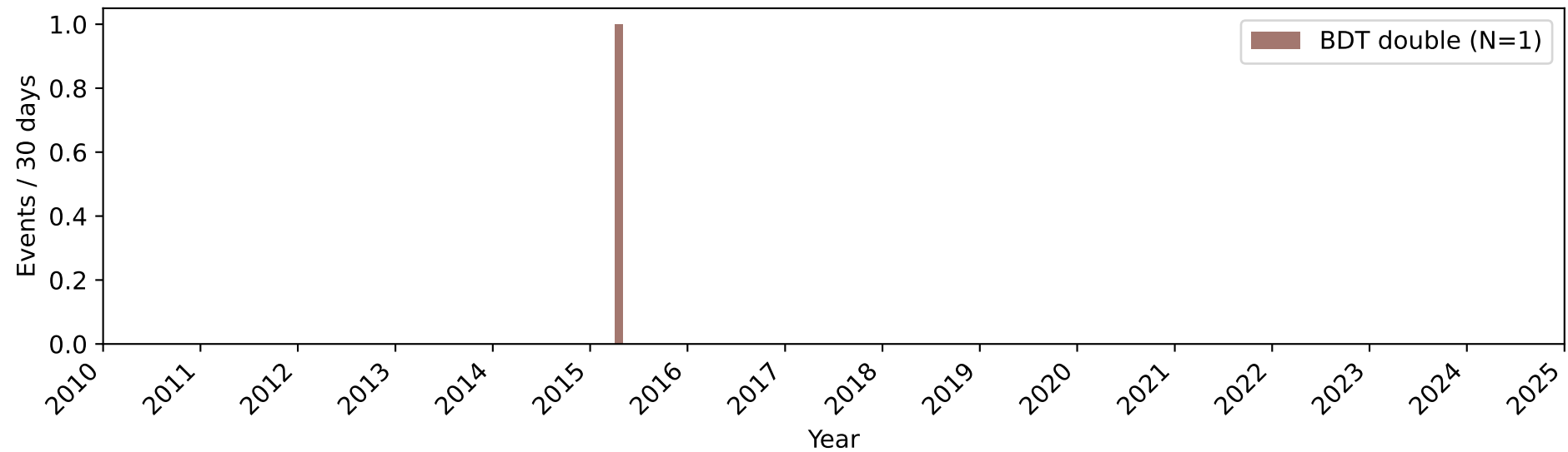
BDT double [E > 60 TeV]
