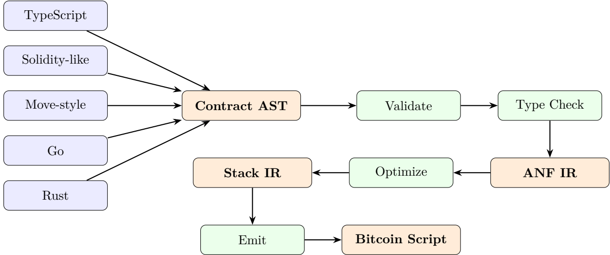
Figure 2: Multi-frontend compilation pipeline. All five frontends converge onto the shared Contract AST; subsequent passes are syntax-agnostic.
