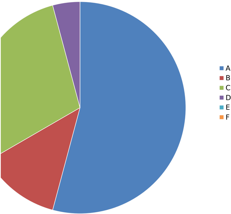
Grade Distribution
