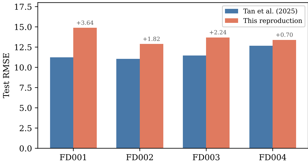
Reproduction vs. reported results (GPT4RUL + condition embedding)
