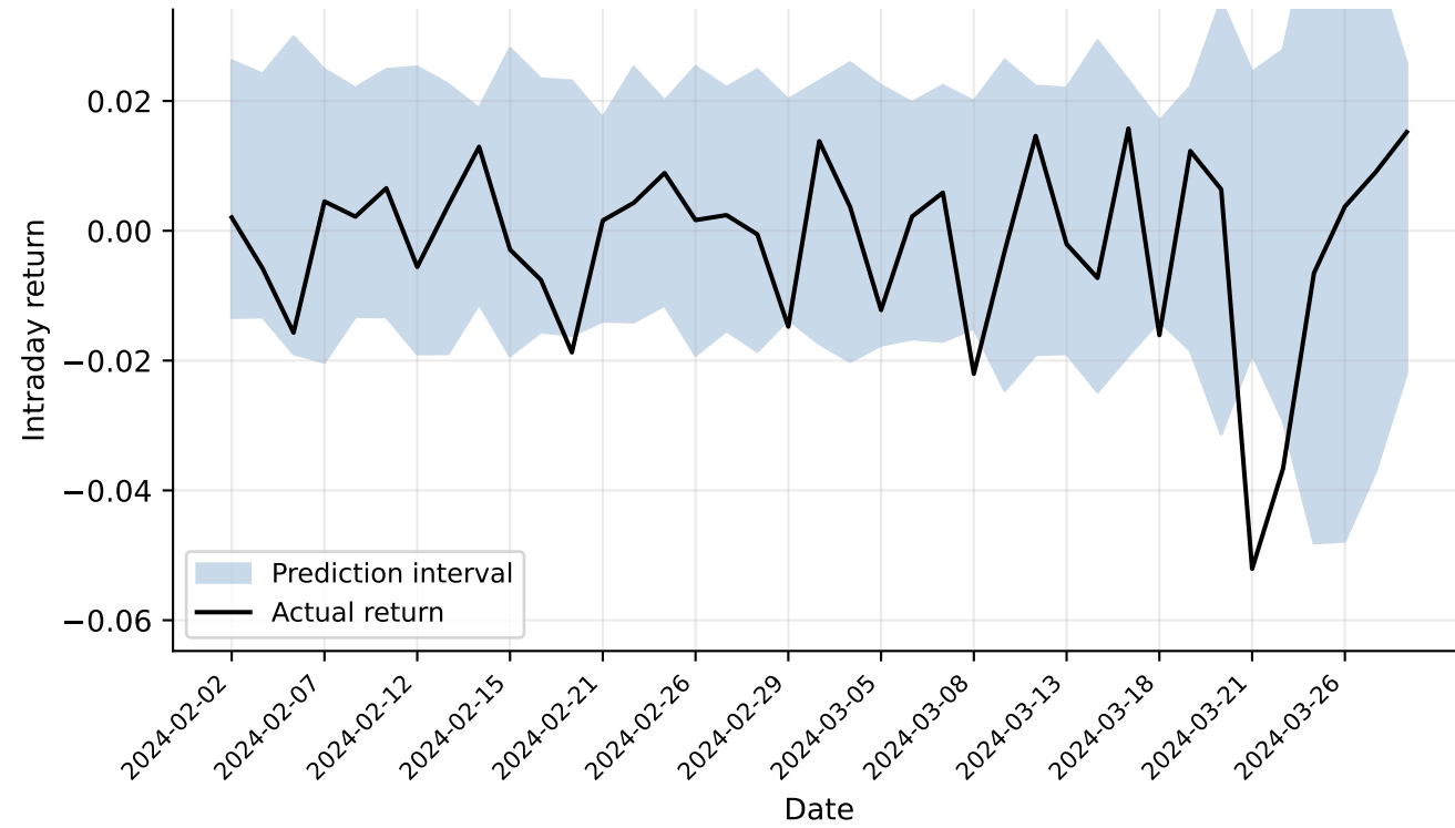
ACN — Return vs. Prediction Interval
