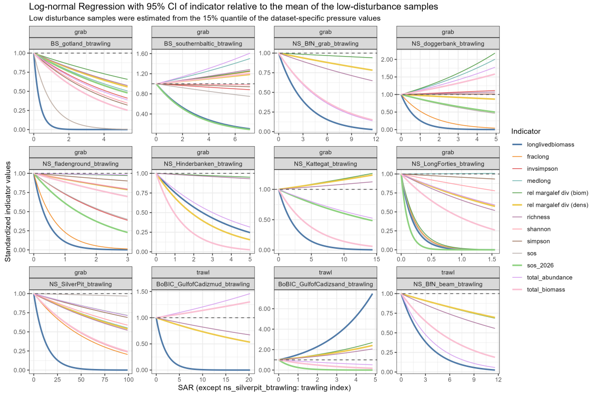
Figure 1: Pressure-state response curves for all indicators.
