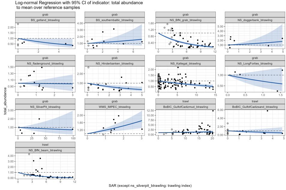
Figure 12: Pressure-state response curves for total abundance.
