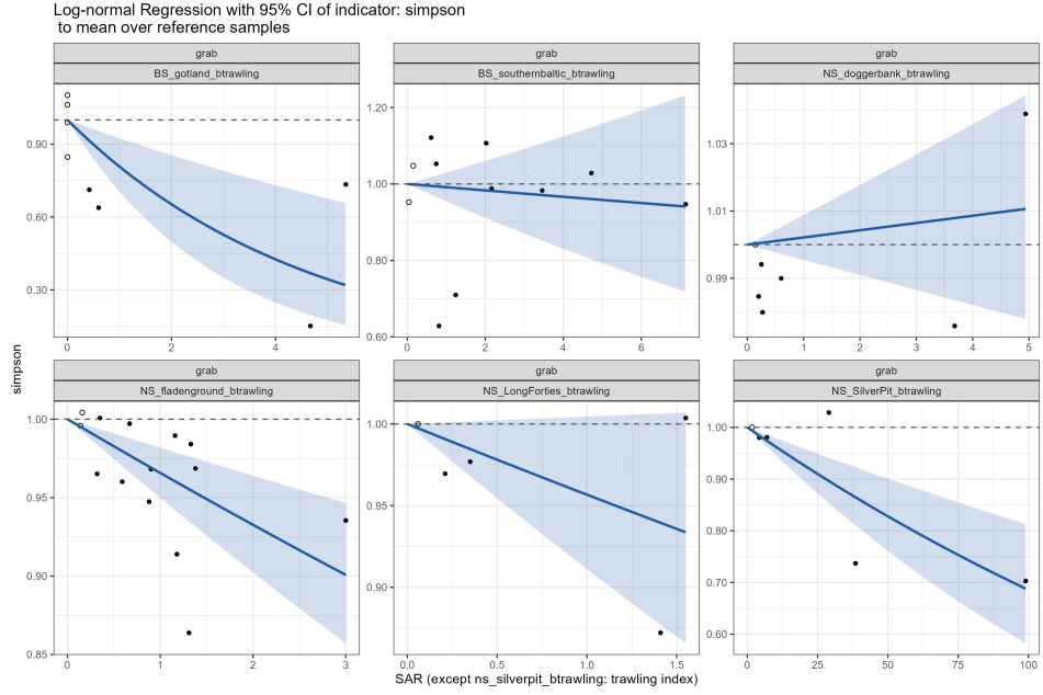
Figure 10: Pressure-state response curves for Simpson diversity.
