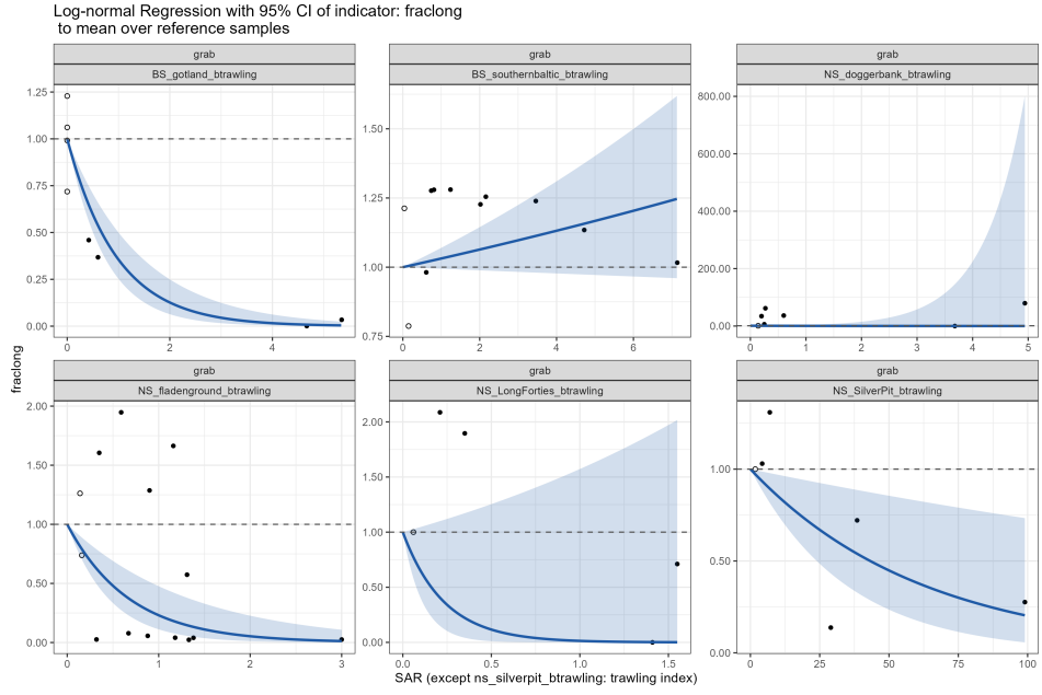
Figure 9: Pressure-state response curves for Fraction long-lived.
