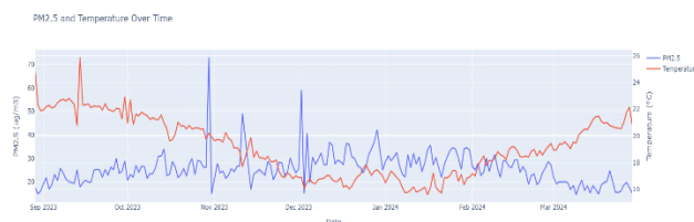
Figure 4. Time Series of Average PM2.5 and Temperature
