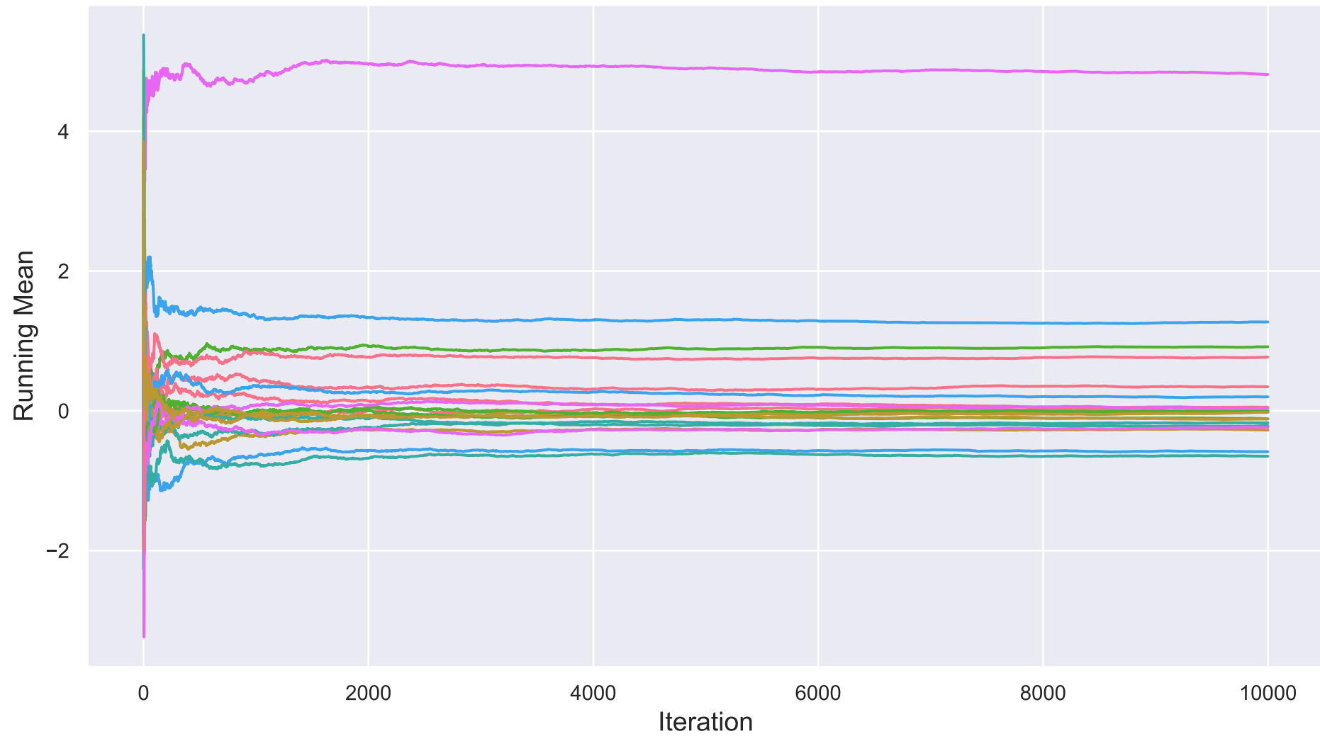
Gibbs
