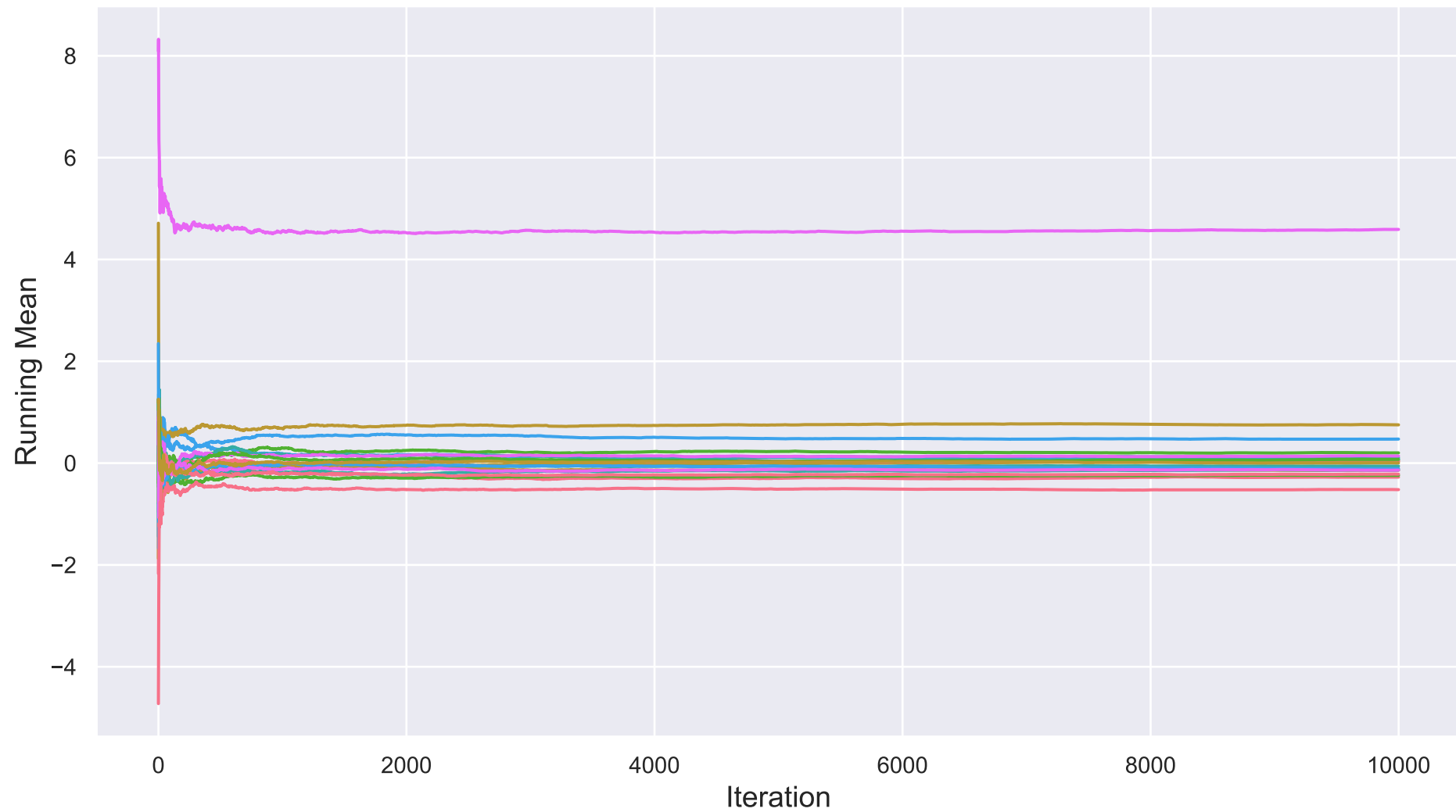
UV-Hadamard
