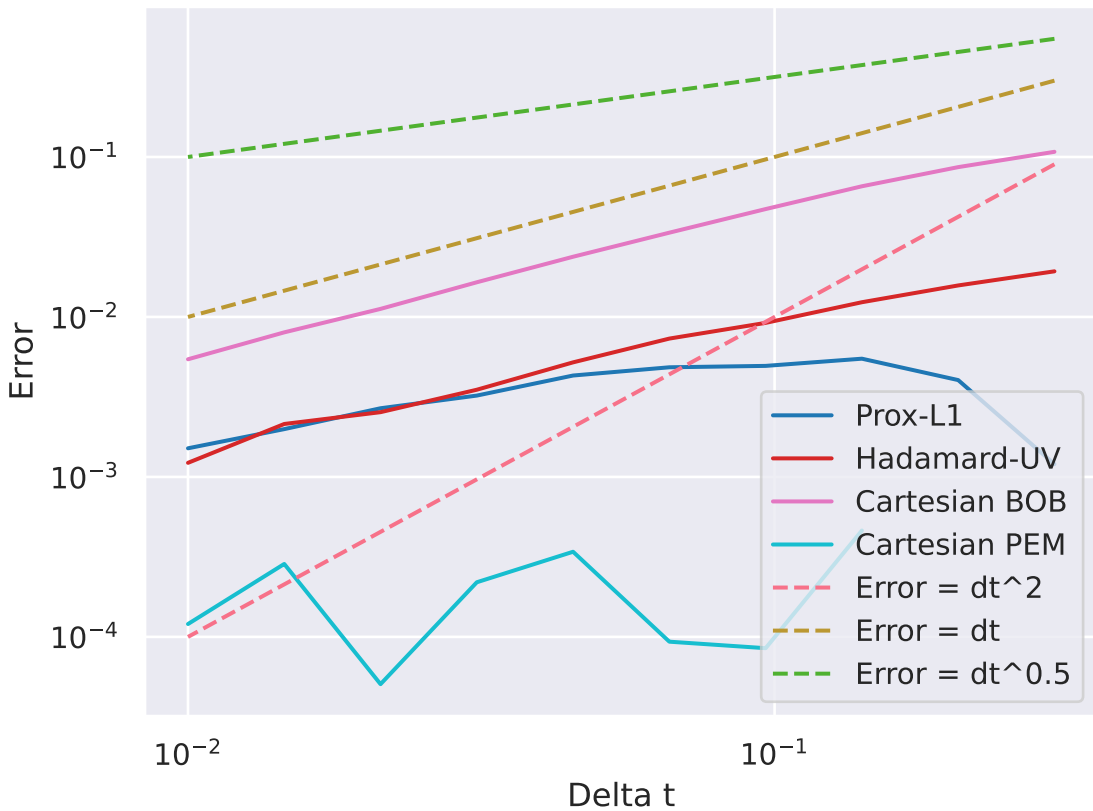
Quadrature error vs stepsize
