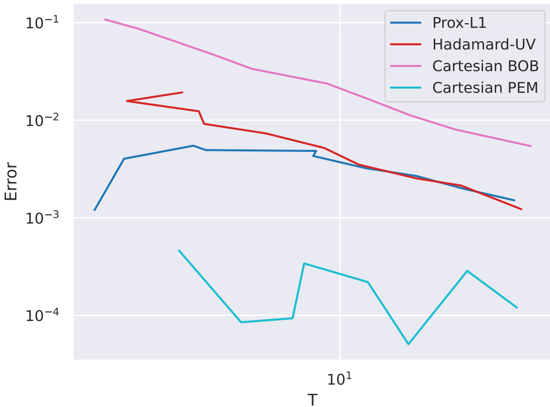
Quadrature error vs burn-in time
