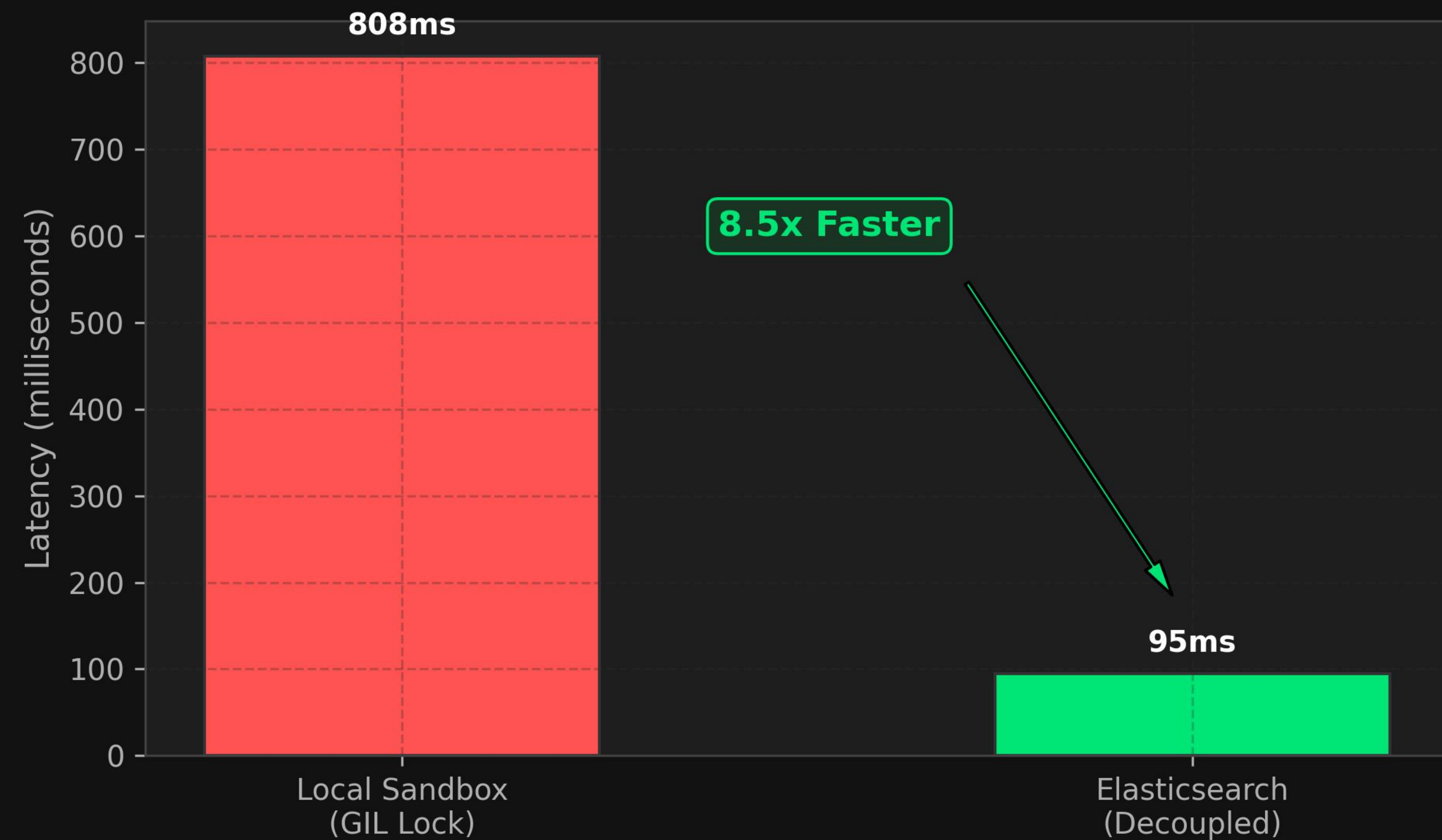
Write Ingestion Lock Time (1,000 Tickets)
