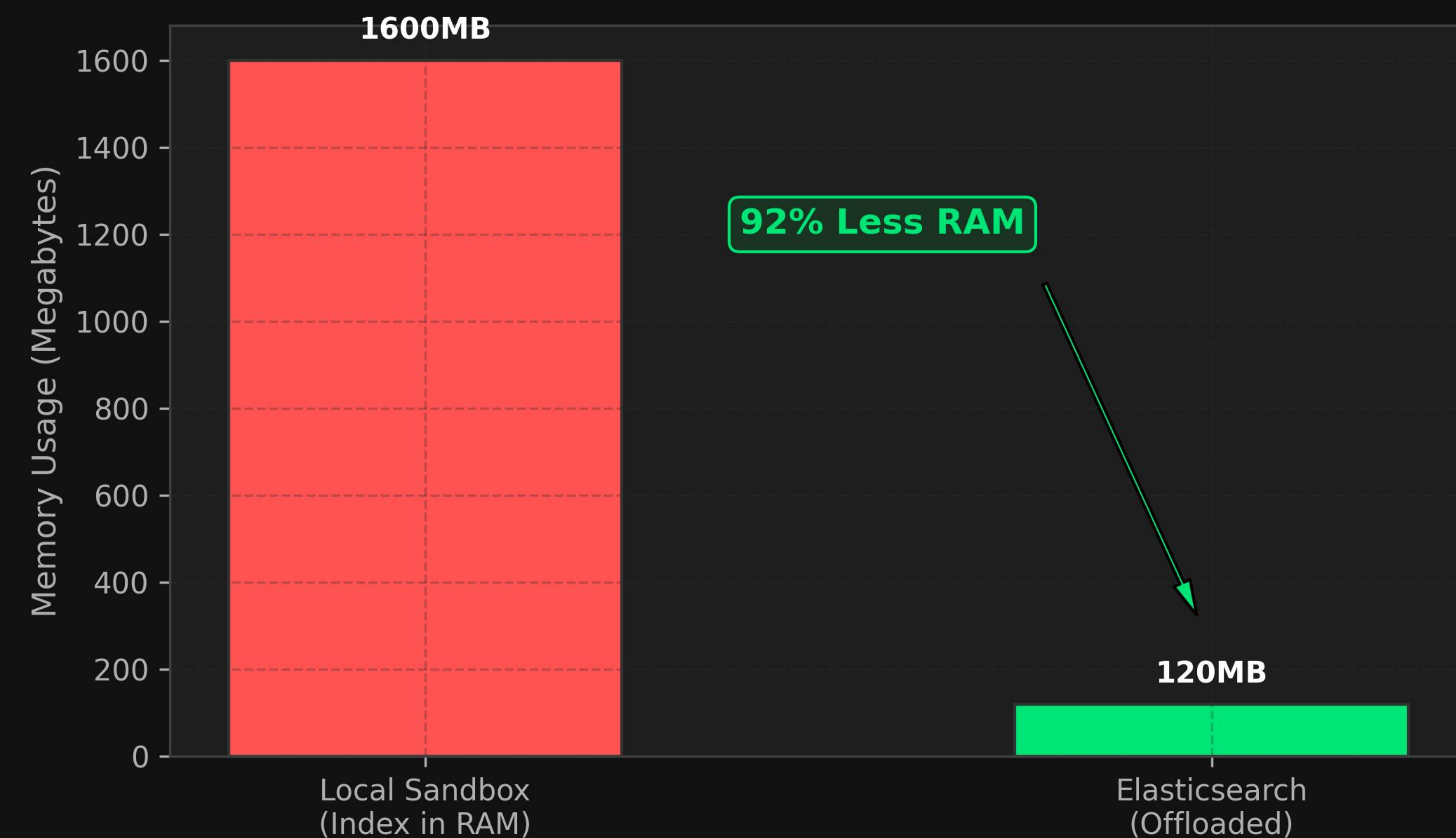
API Process Memory Footprint
