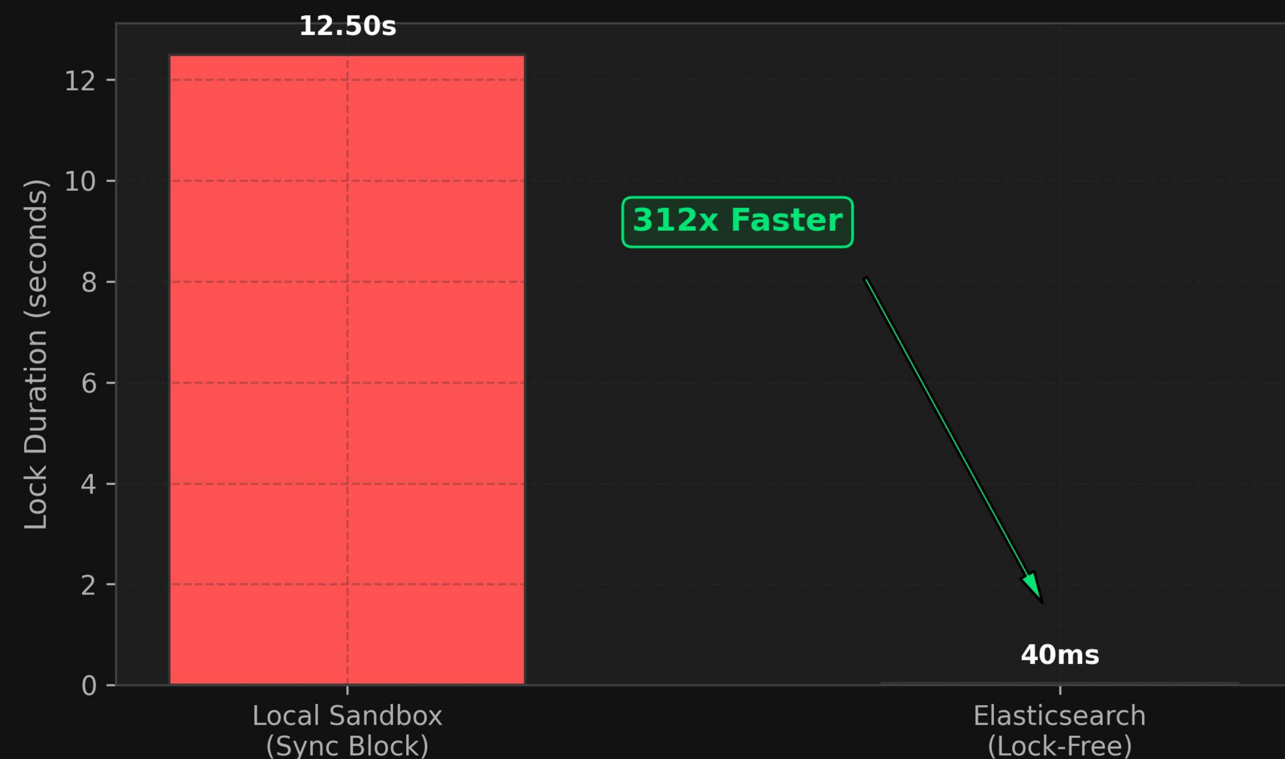
Write Ingestion Lock Time (1,000 Tickets)
