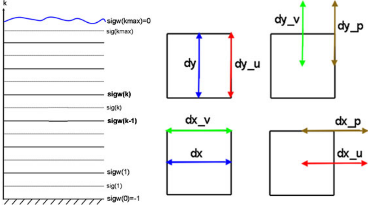
Figure 11.10: MARS grid structure.
