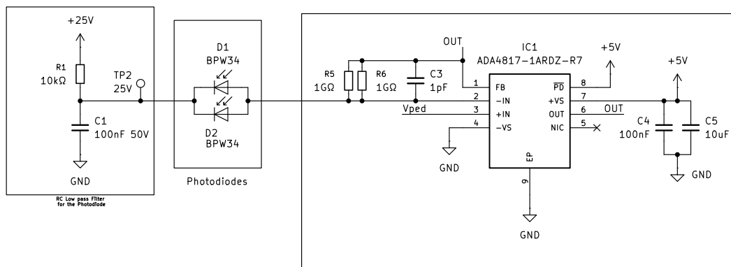
Charge Amplifier
