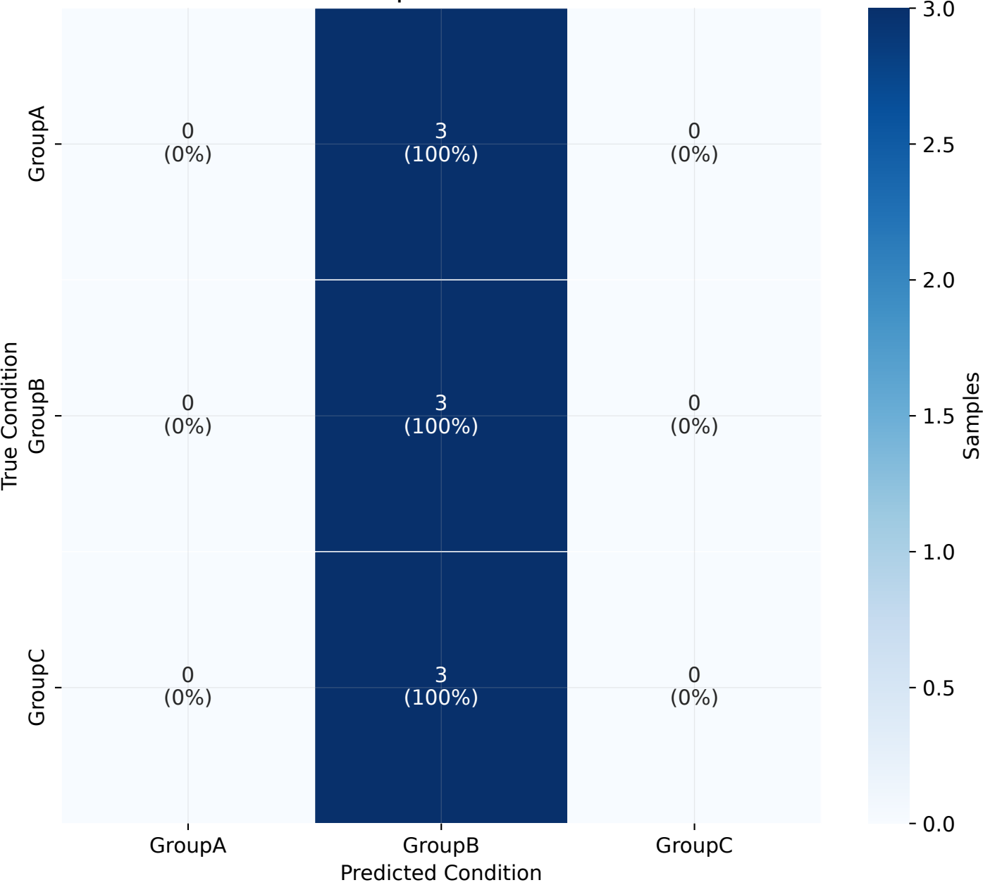
Confusion Matrix F1 (macro) = 0.17 | ROC-AUC (macro) = 0.52
