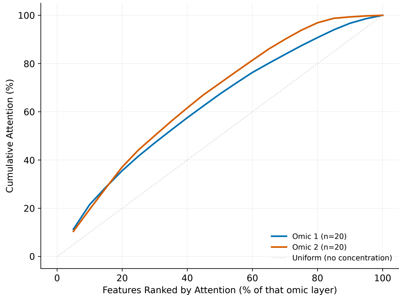
Attention Concentration: Omic 1 vs. Omic 2
