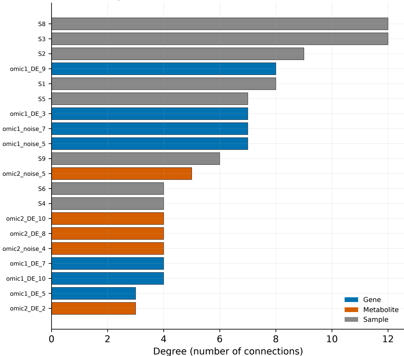
Top 20 Hub Nodes in the Attention Network
