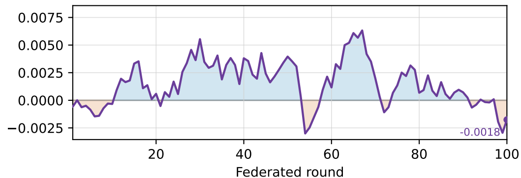
Method gap: CKKS+Skeleton – SHE-LoRA (CKKS)
