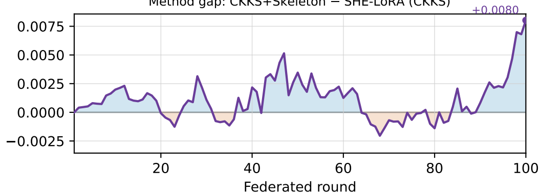
Method gap: CKKS+Skeleton – SHE-LoRA (CKKS)
