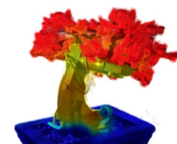
Poisson's ratio
