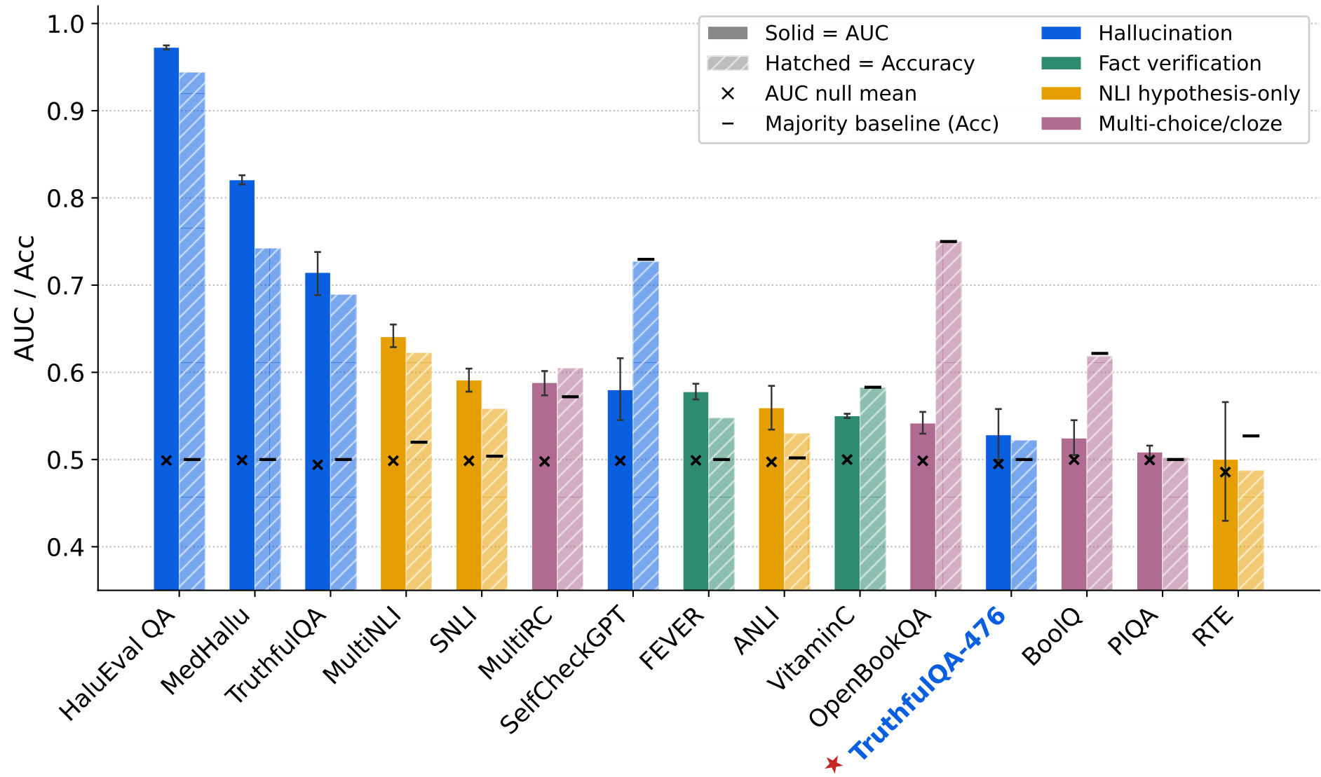
Cross-dataset surface-form audit (SURFACE6)
