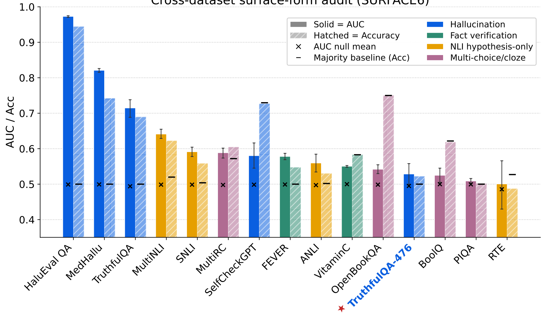
Cross-dataset surface-form audit (SURFACE6)
