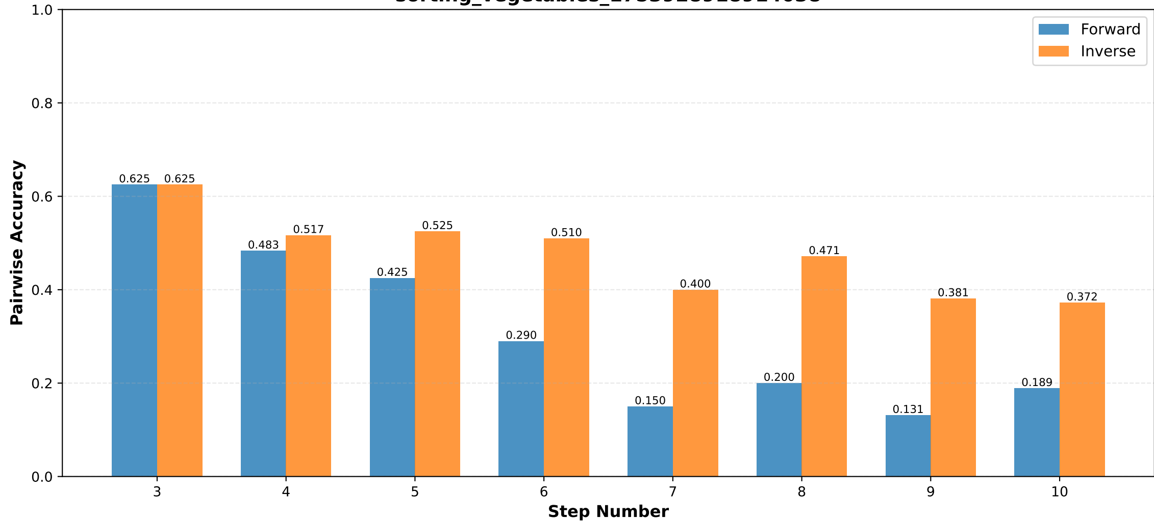
Pairwise Accuracy by Step Number sorting_vegetables_1753928918914038
