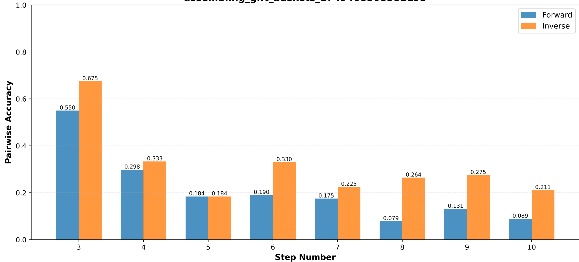
Pairwise Accuracy by Step Number assembling_gift_baskets_1749468508582193
