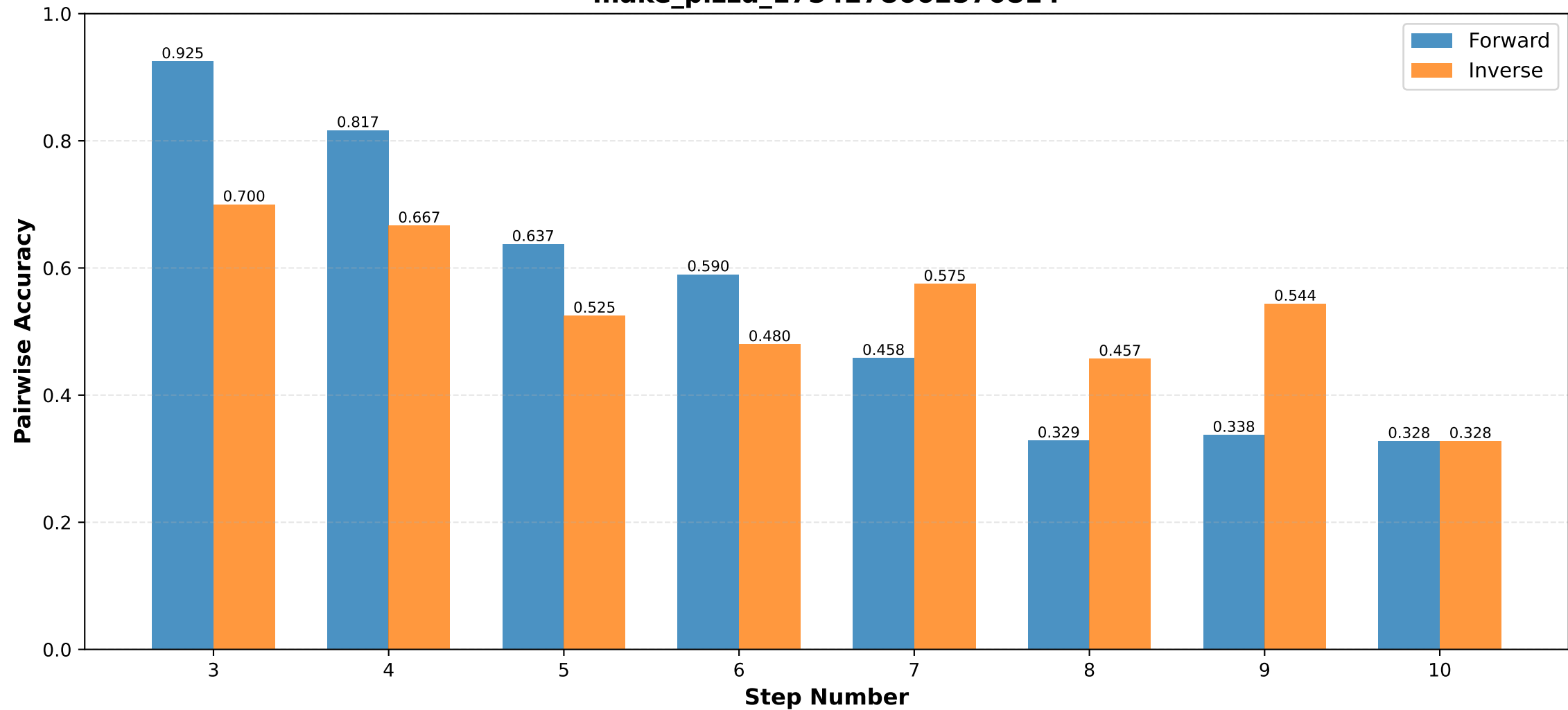
Pairwise Accuracy by Step Number make_pizza_1754278662570814
