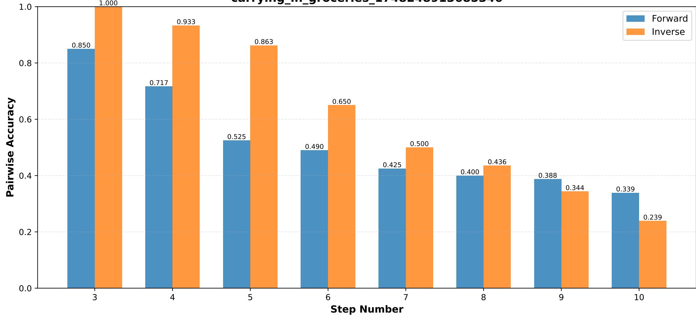
Pairwise Accuracy by Step Number carrying_in_groceries_1748248913685346
