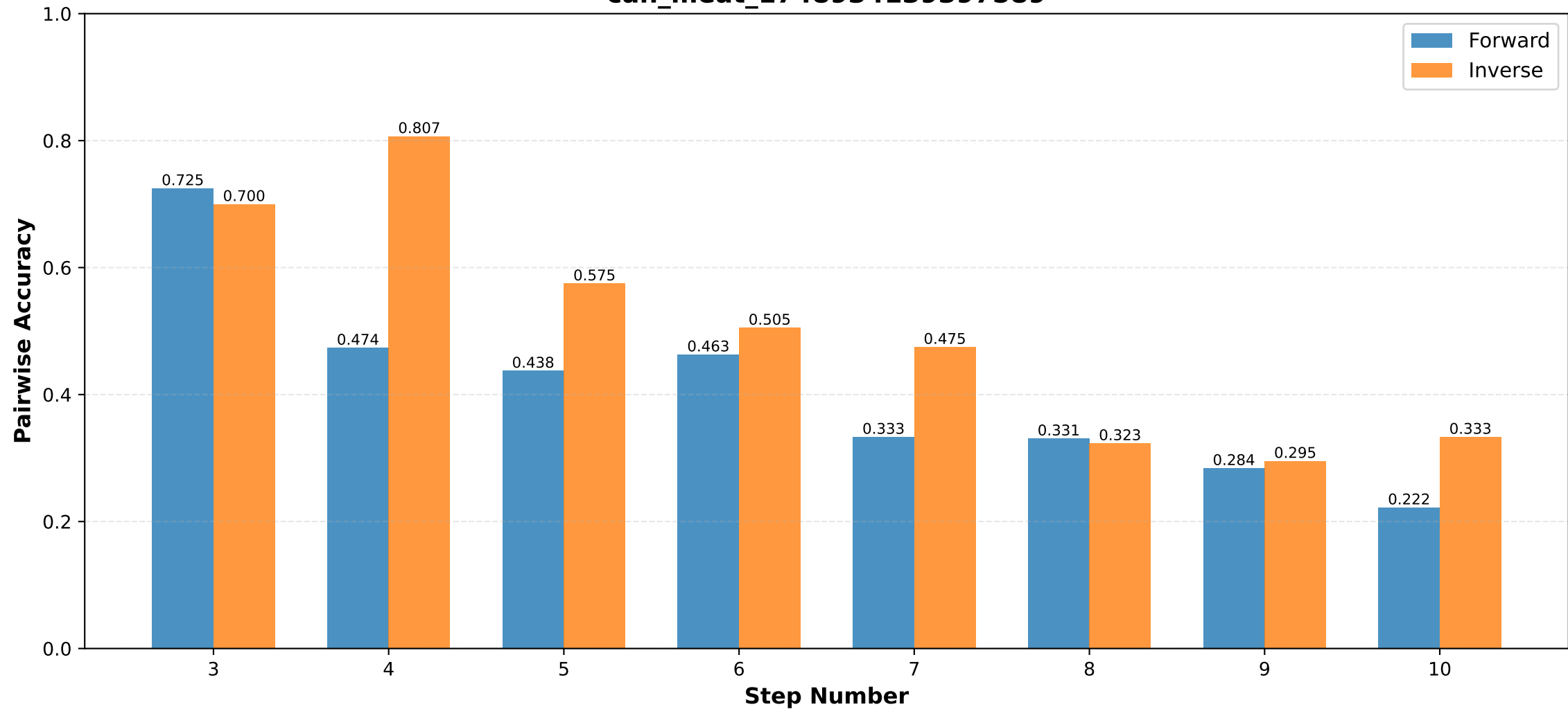
Pairwise Accuracy by Step Number can_meat_1748934139397589
