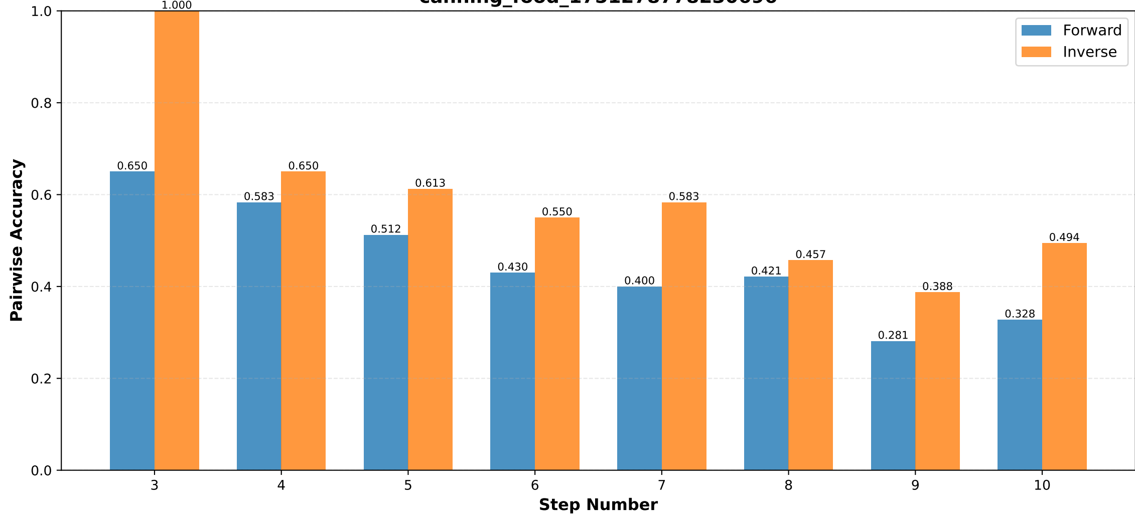
Pairwise Accuracy by Step Number canning_food_1751278778230696
