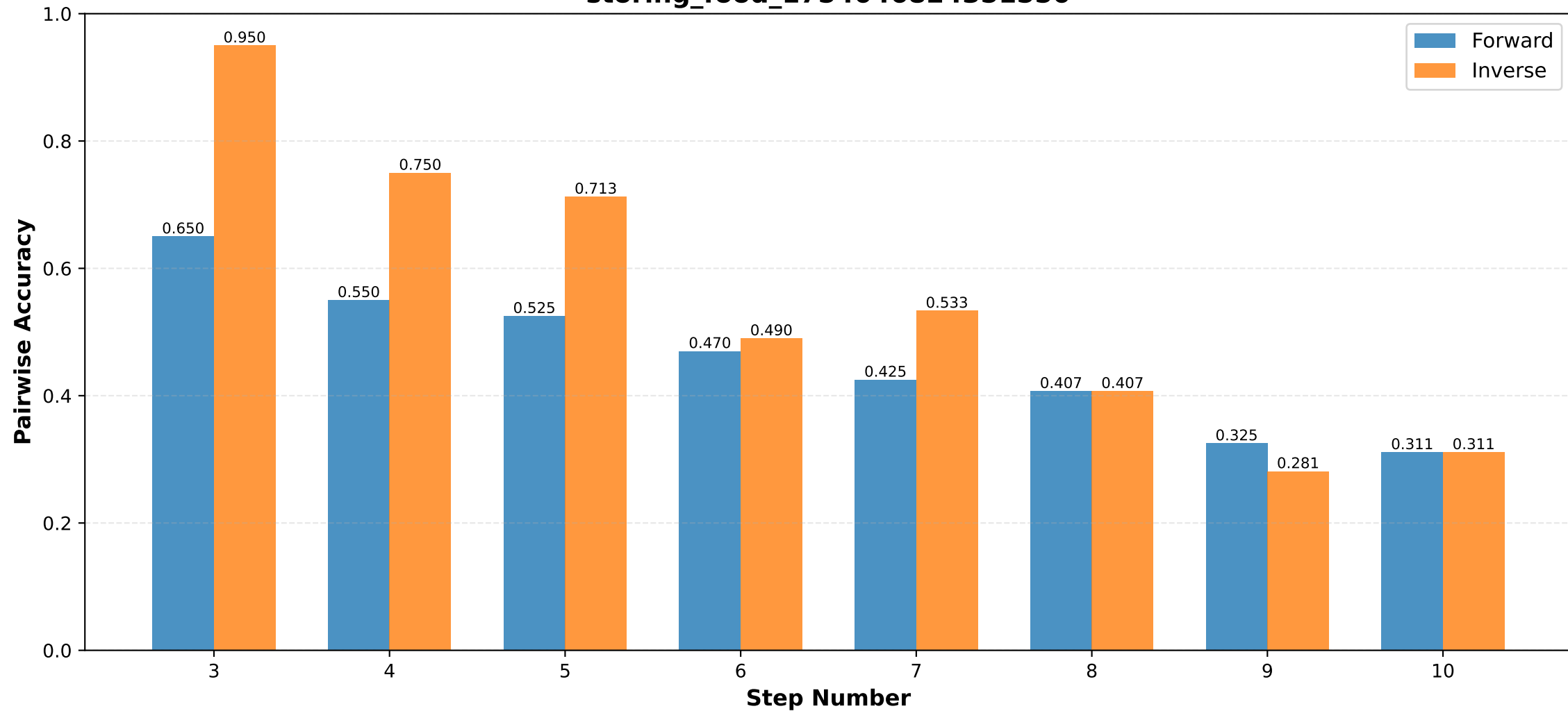
Pairwise Accuracy by Step Number storing_food_1754046824351550
