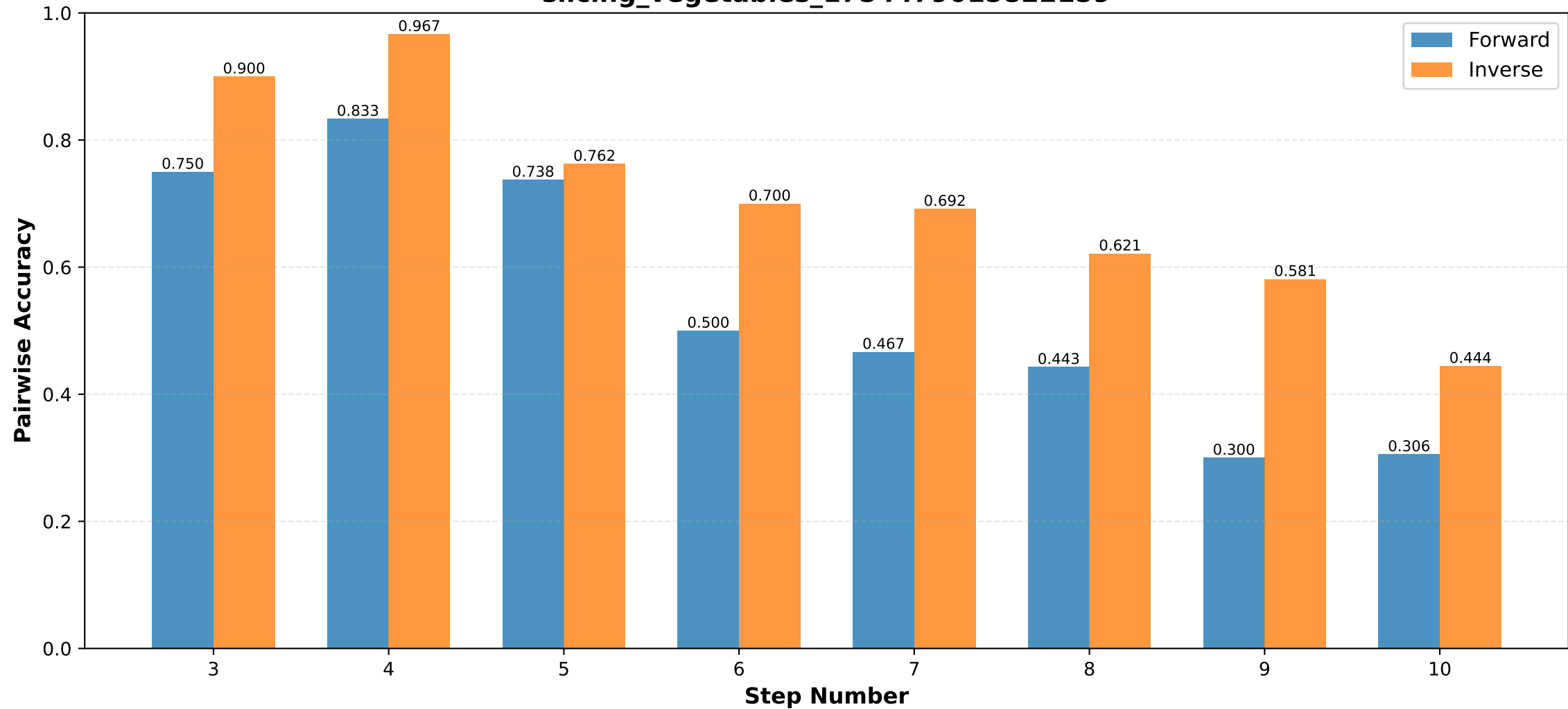
Pairwise Accuracy by Step Number slicing_vegetables_1754479015822159
