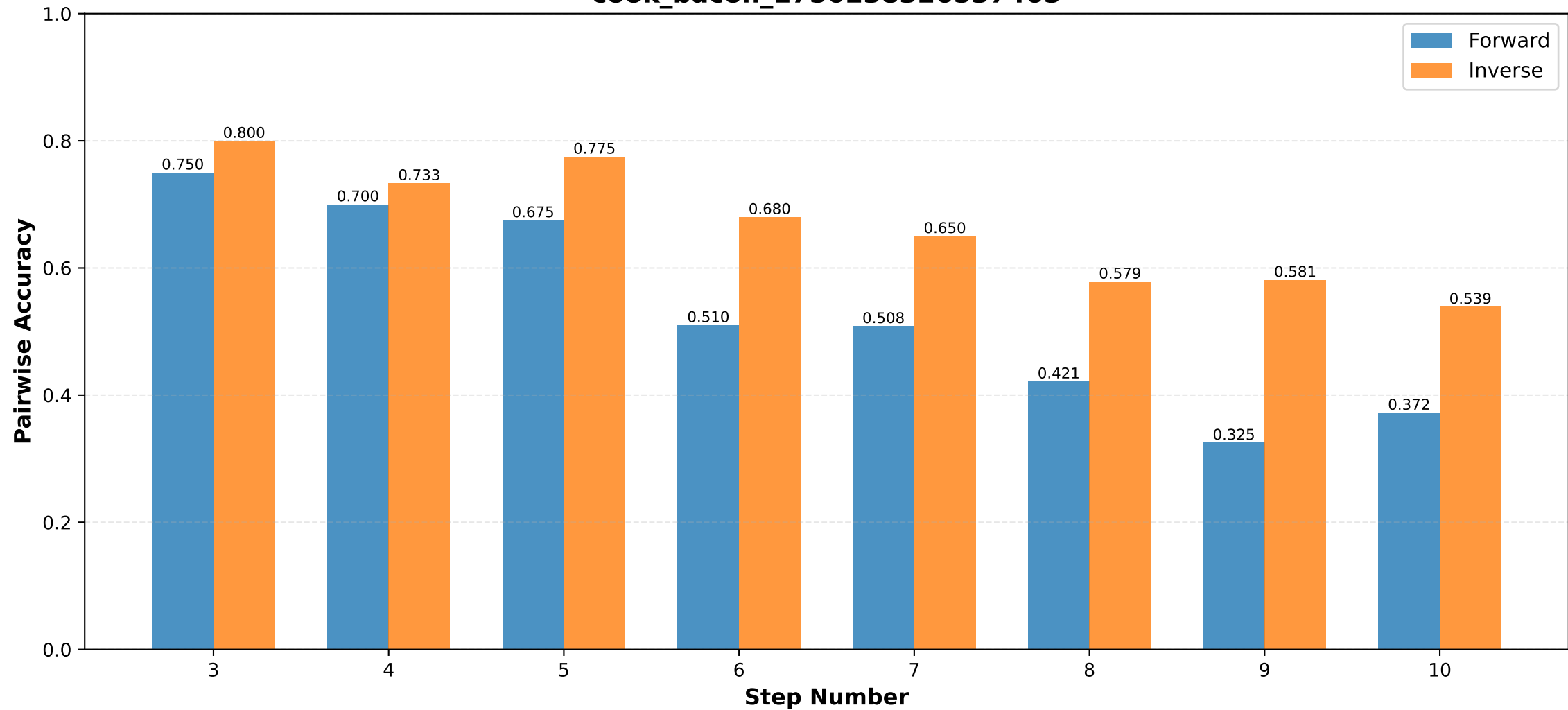
Pairwise Accuracy by Step Number cook_bacon_1750238326537465
