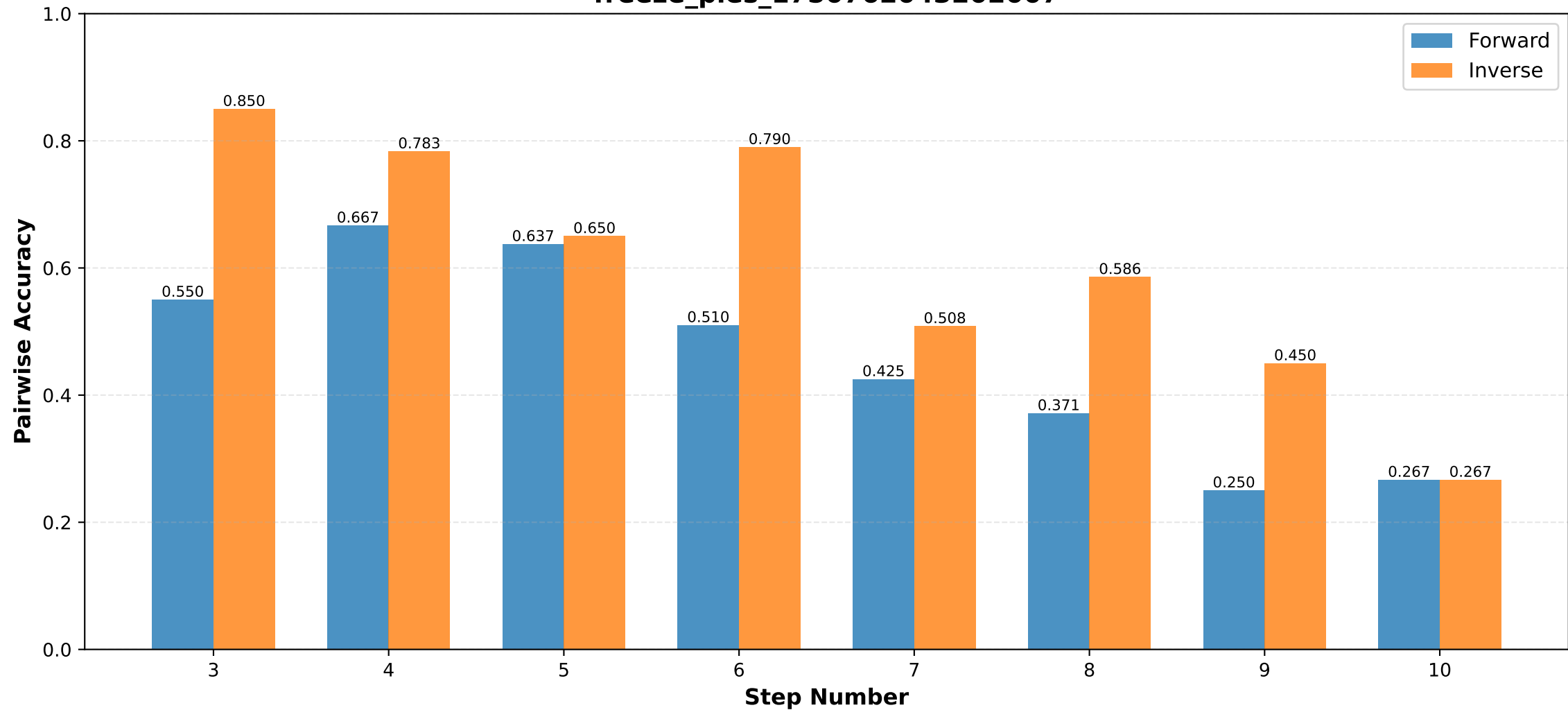
Pairwise Accuracy by Step Number freeze_pies_1750762043202007
