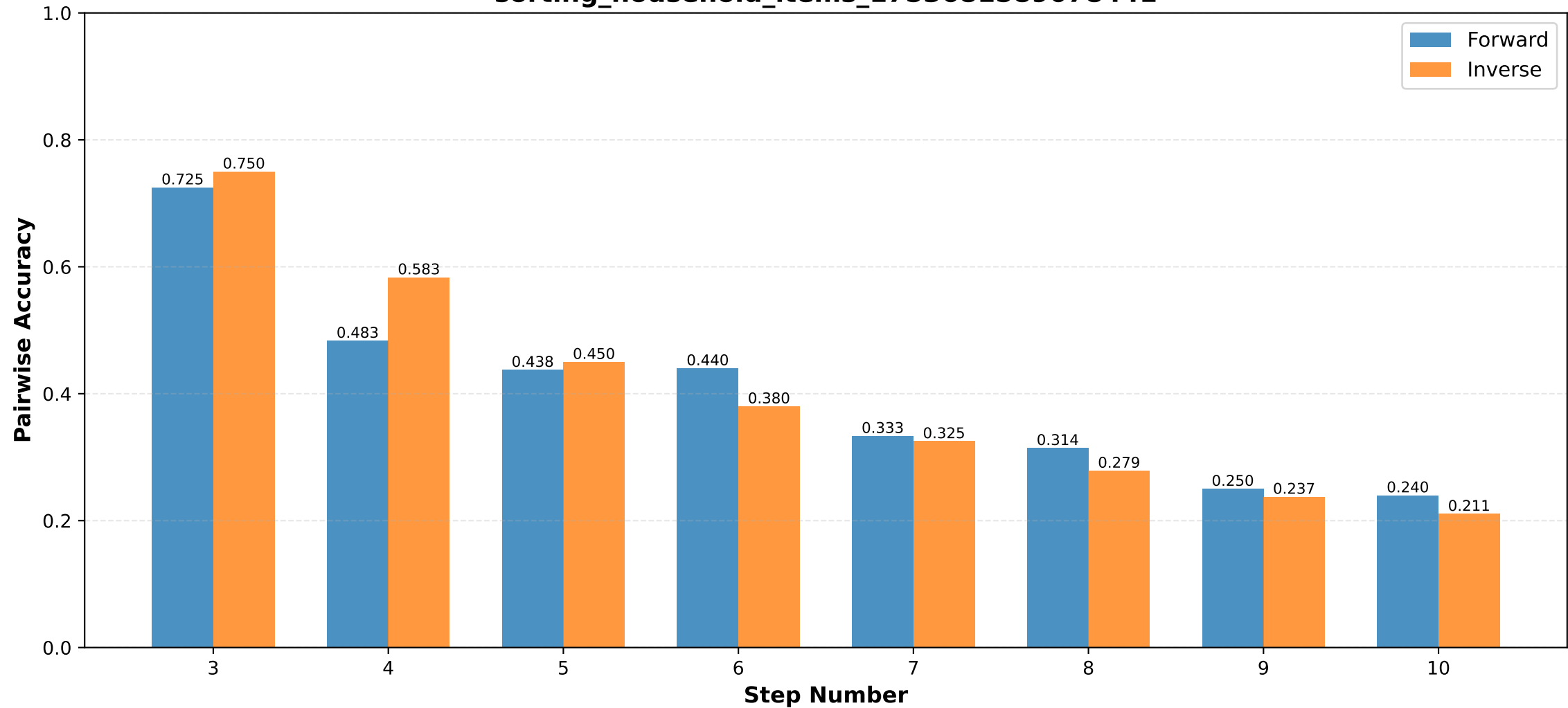
Pairwise Accuracy by Step Number sorting_household_items_1753681589078441
