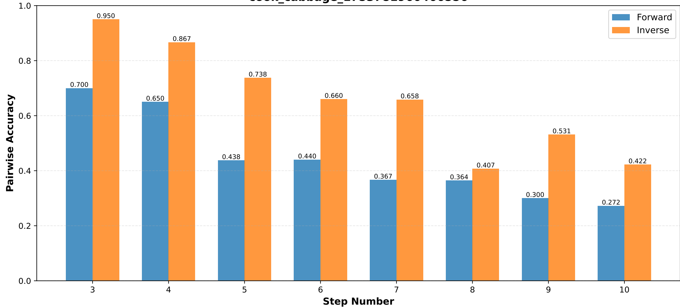
Pairwise Accuracy by Step Number cook_cabbage_1753781960466556
