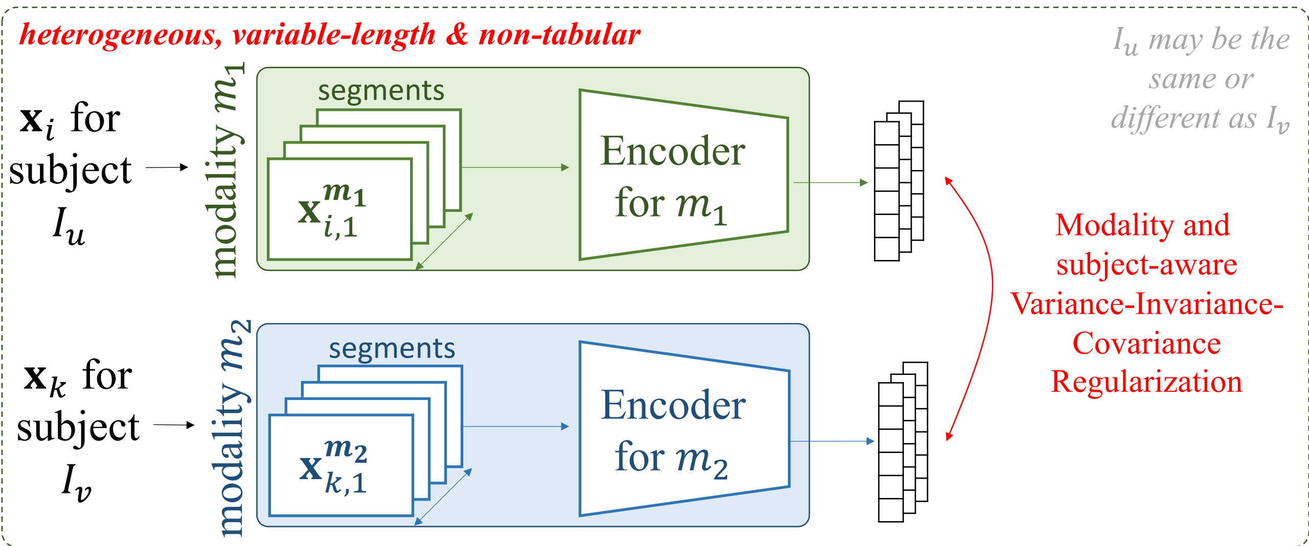
(c) FairSSL : SSL for heterogeneous, variable-length, non-tabular, multimodal data with subject-aware and modality-aware variance-invariance-covariance regularization.
