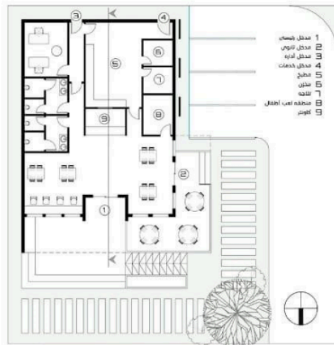
plan scale (1:500)
