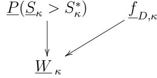
Figure 3: bnet for calculating warning W_\kappa
