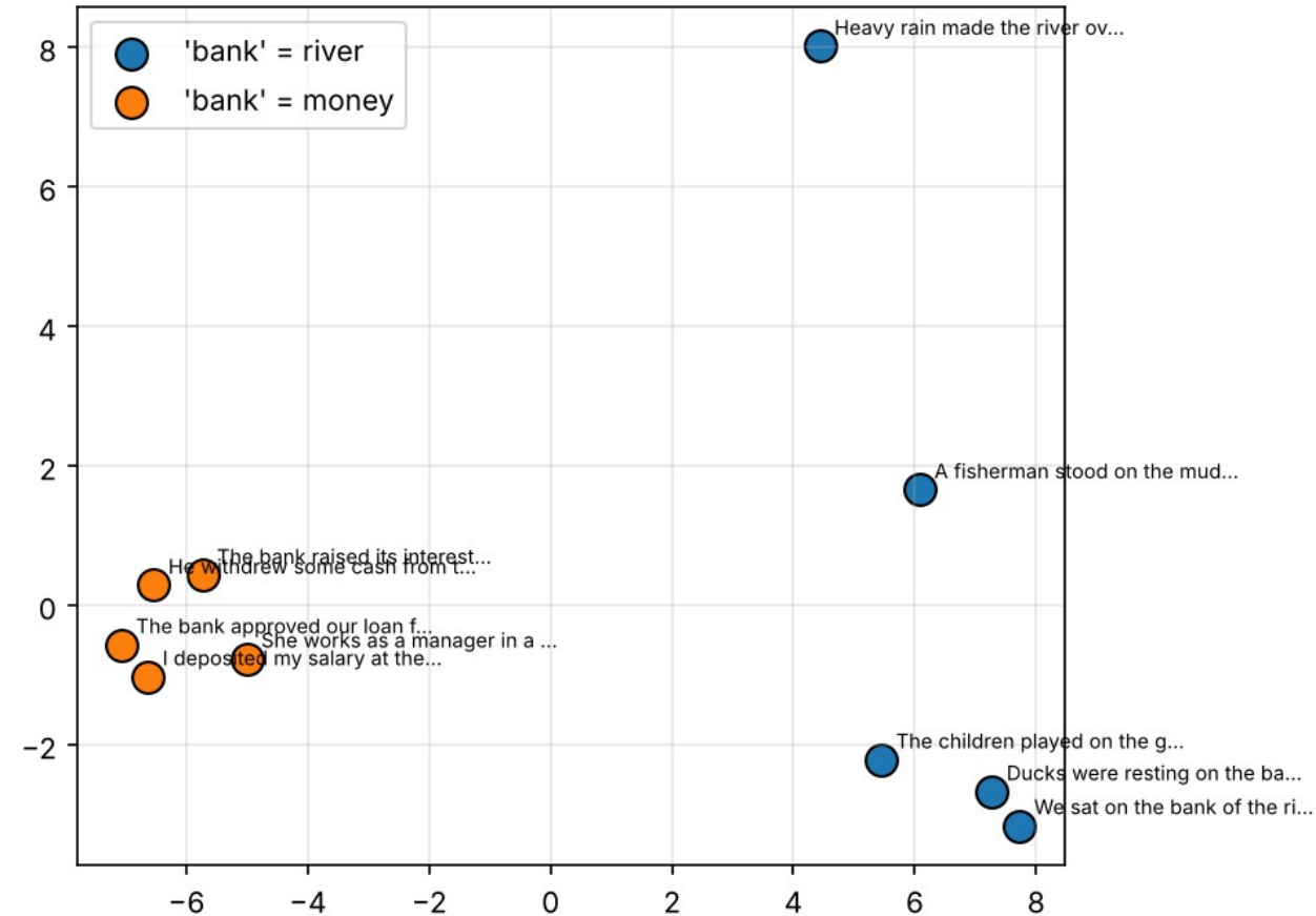
Layer 12 (last layer) PCA keeps 62% of the variance
