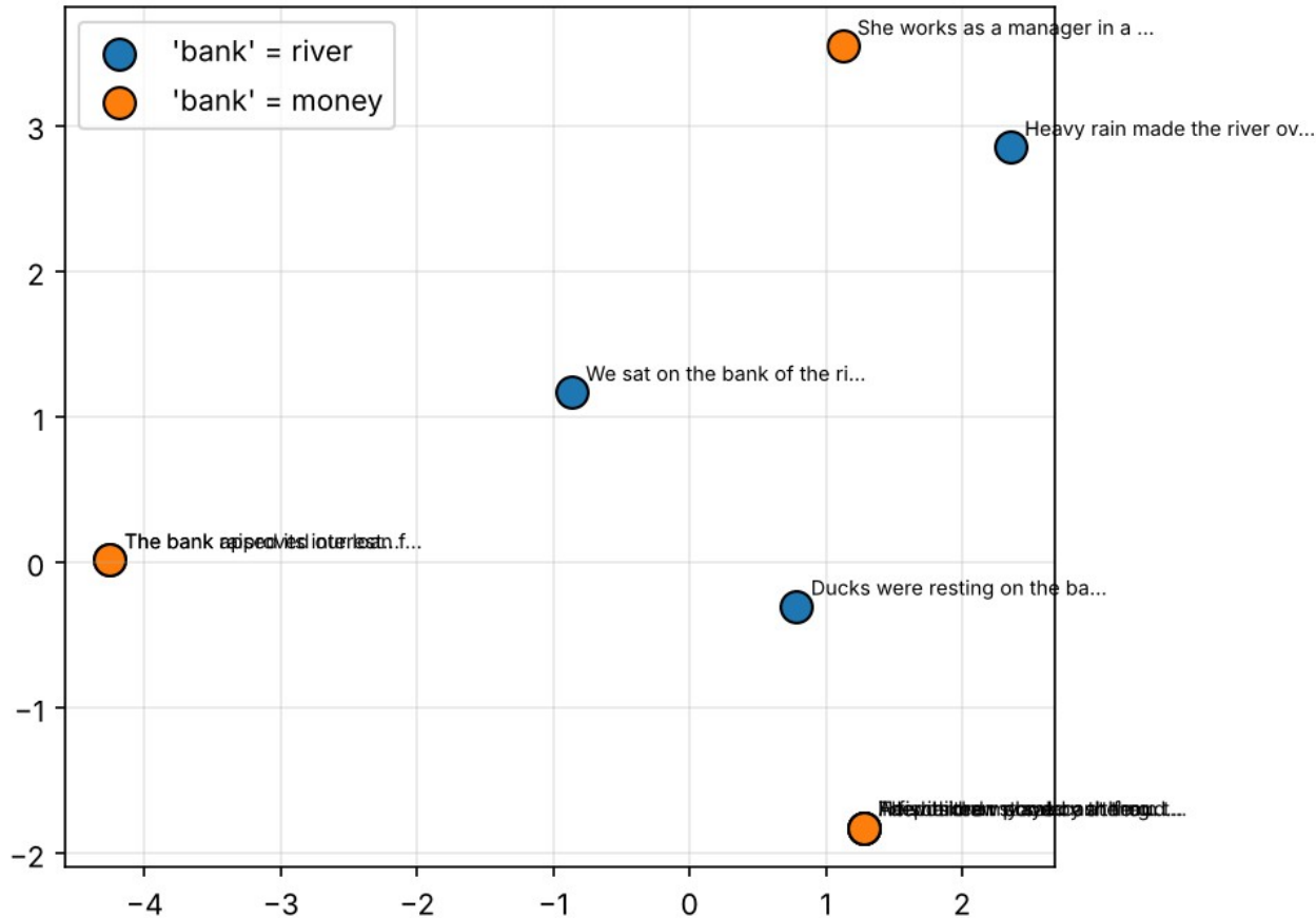
Layer 0 (input embeddings) PCA keeps 71% of the variance
