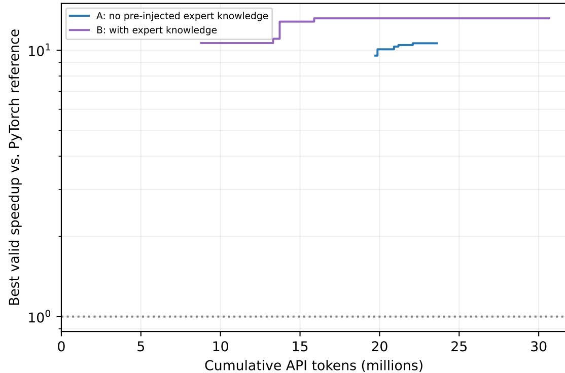
fused_add_rmsnorm
