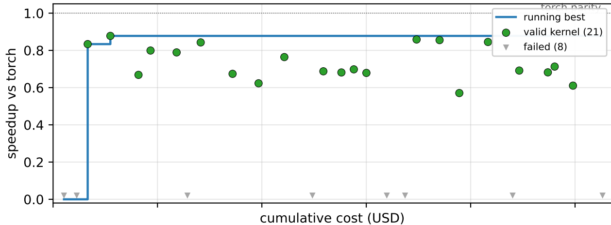
(b) Conv2d: fallback wrappers hide two slow kernels
