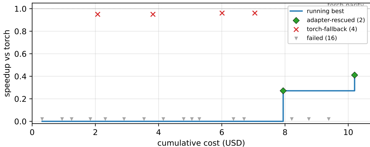
(b) Conv2d: fallback wrappers hide two slow kernels
