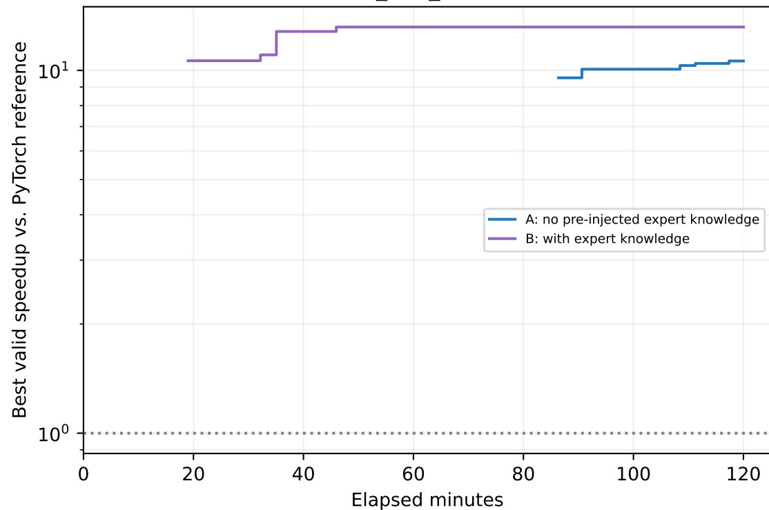
fused_add_rmsnorm
