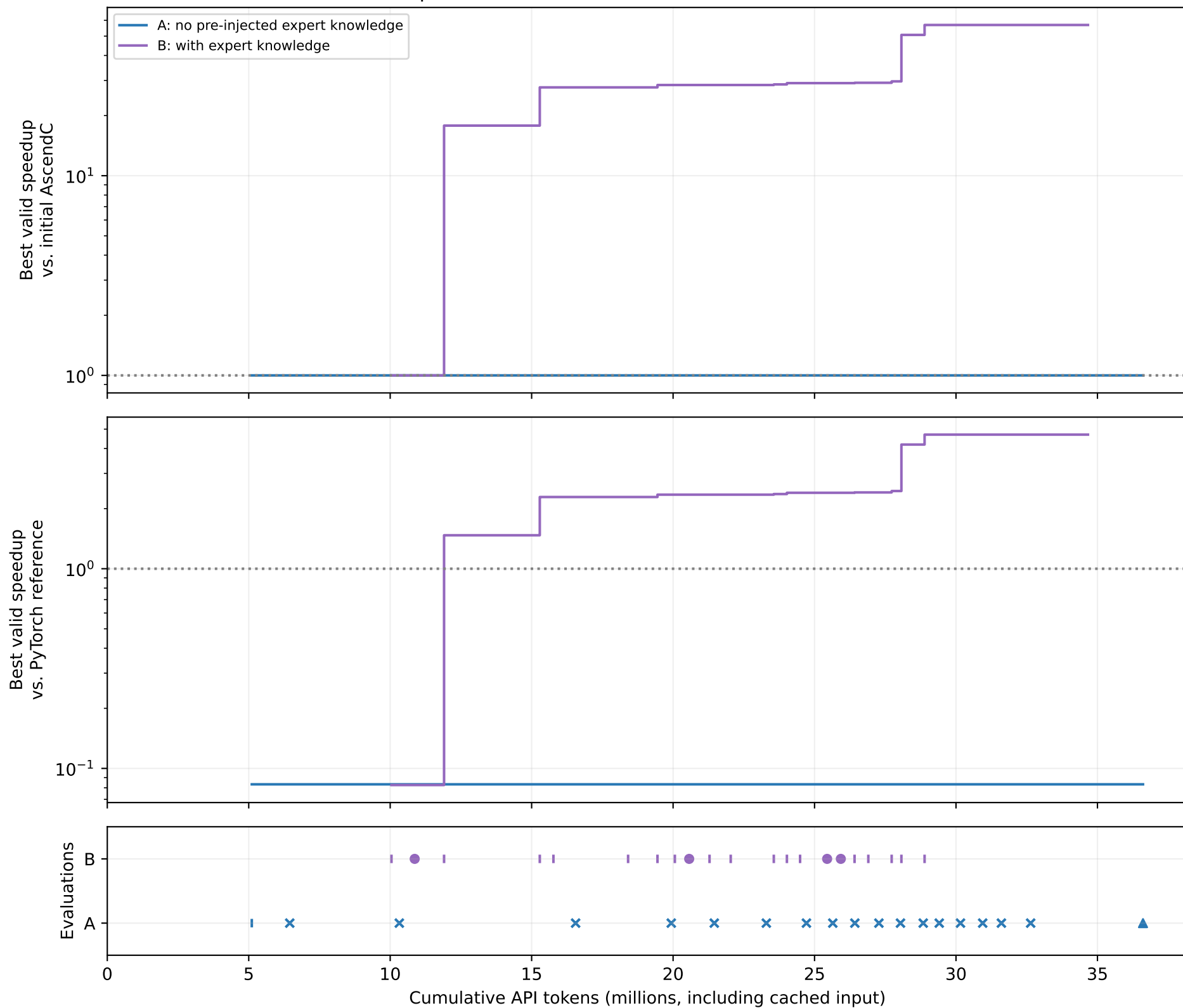
SparseAttention / AscendC / same initial source
