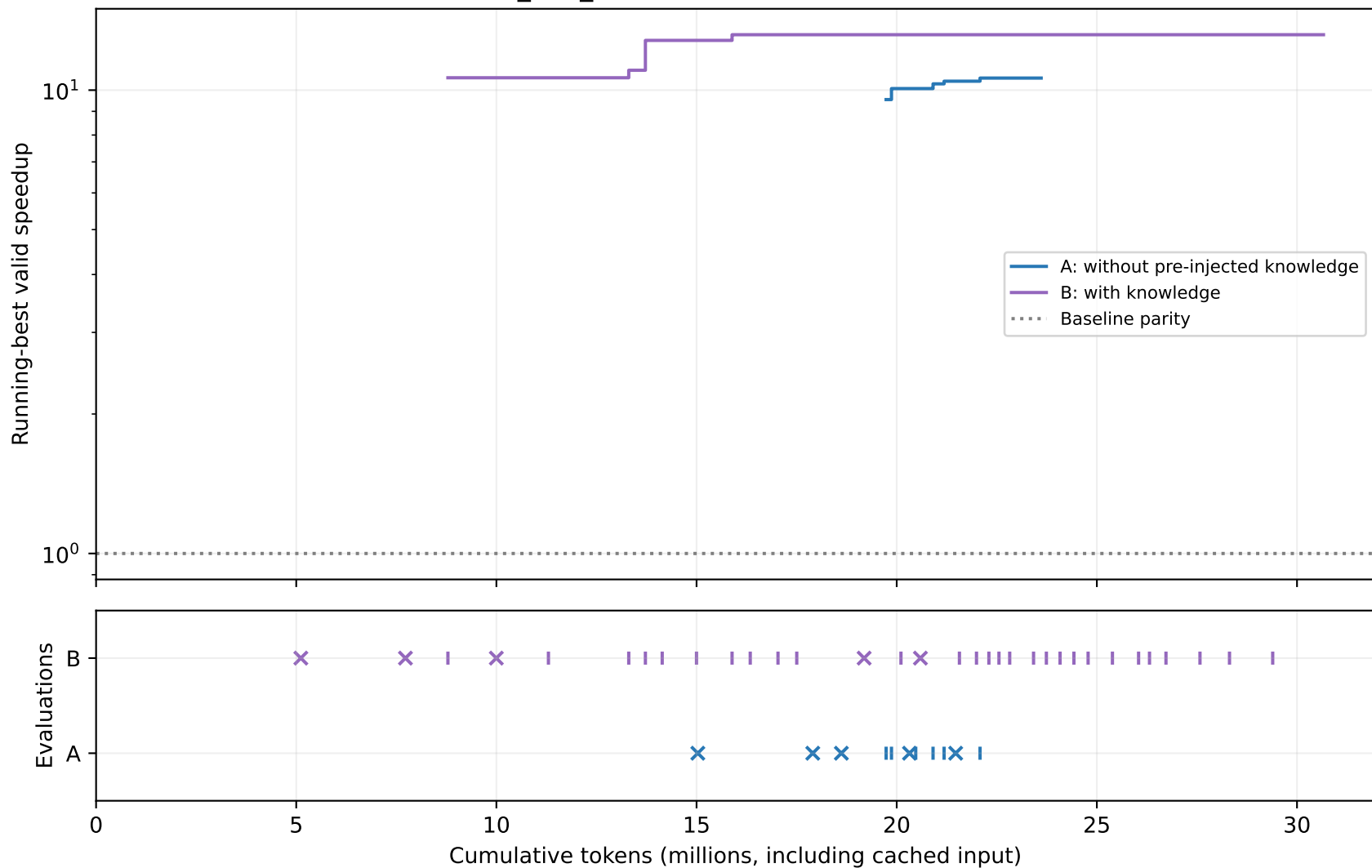
fused_add_rmsnorm — formal AscendC runs
