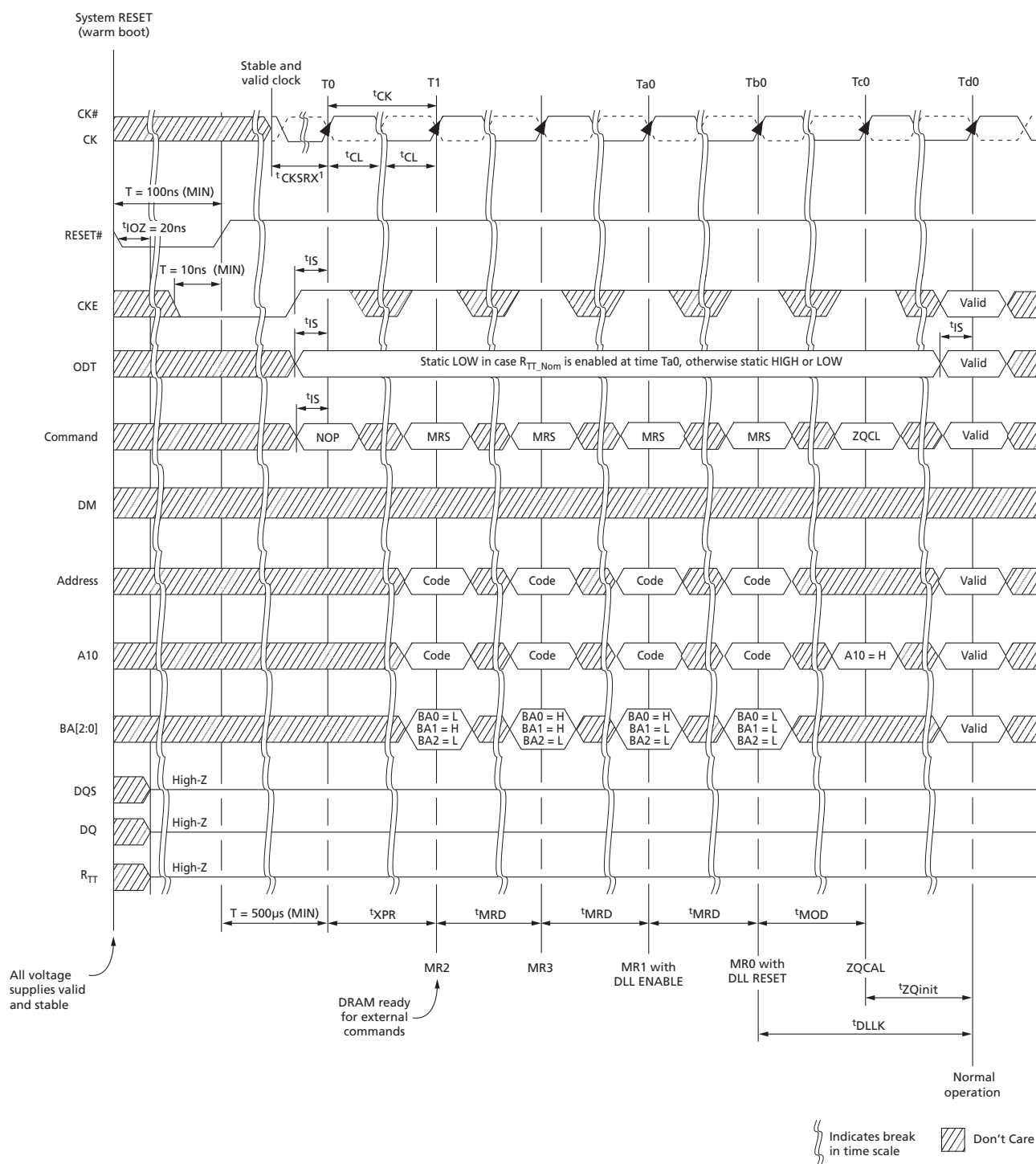
Figure 105: RESET Sequence
