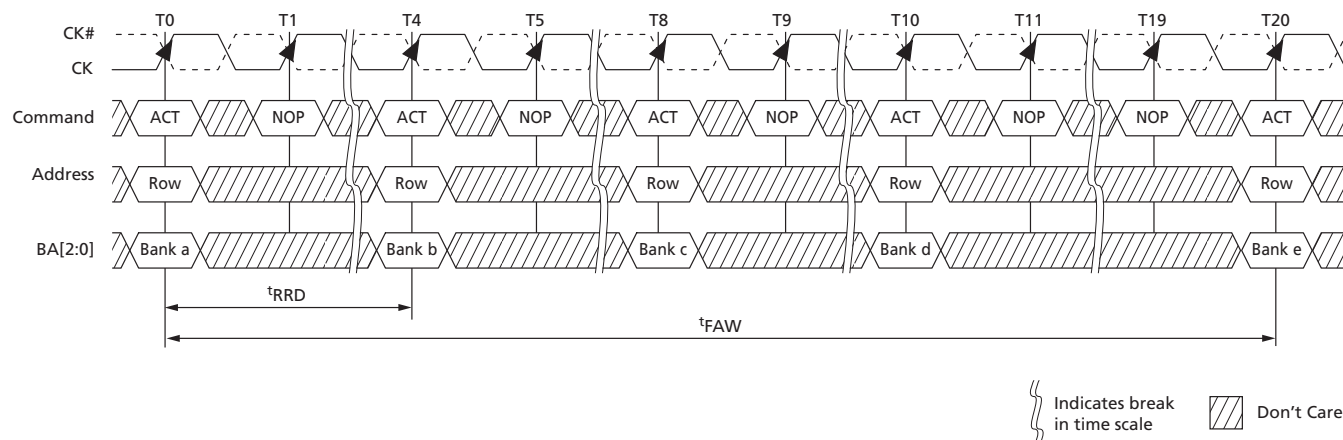
Figure 64: Example: t_{FAW}
