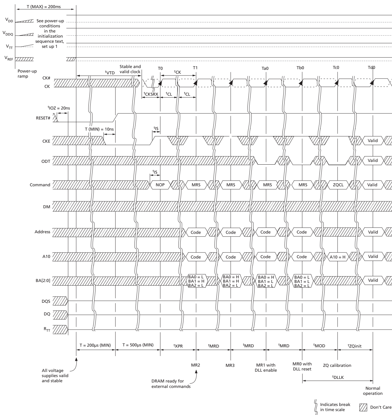
Figure 46: Initialization Sequence
