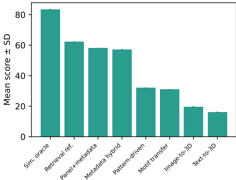
Ten-seed stability
