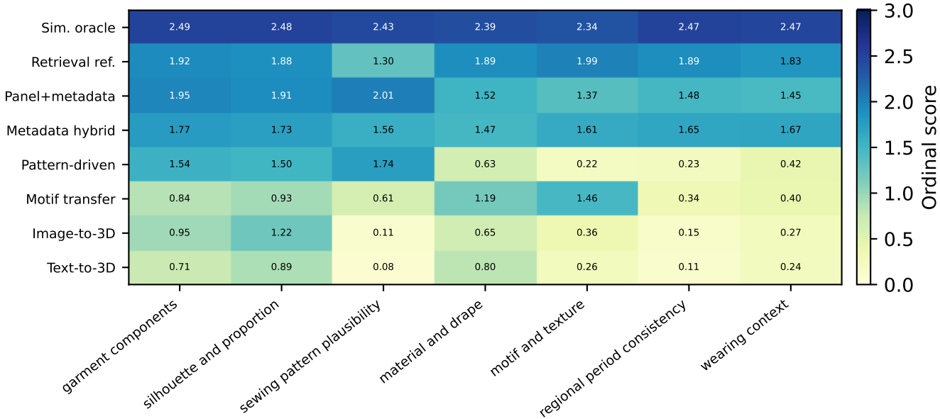
Criterion-level behavior
