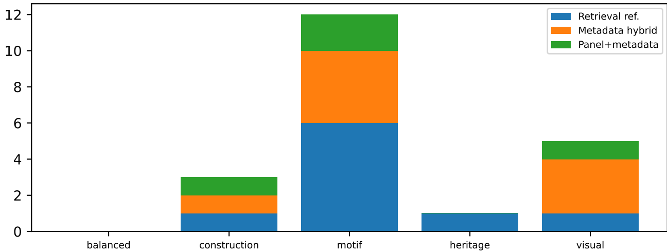
Non-oracle wins
