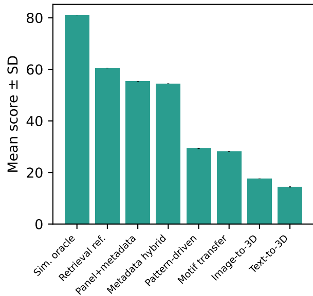
Ten-seed stability
