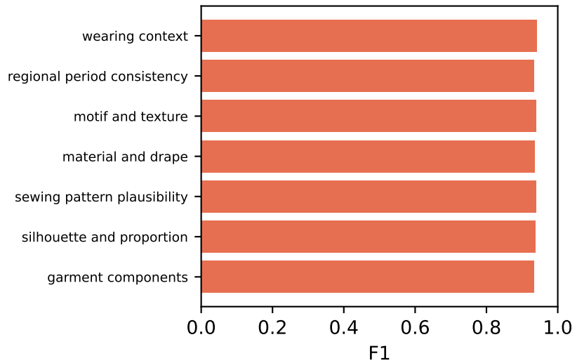
Injected-failure recovery
