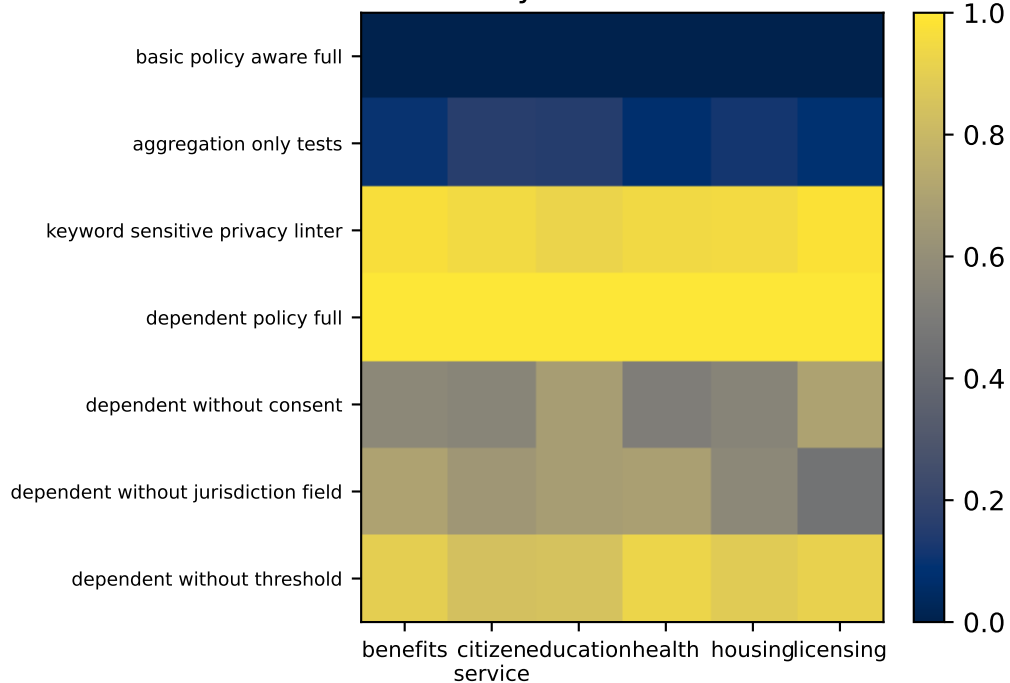
Violation recall by method and service domain
