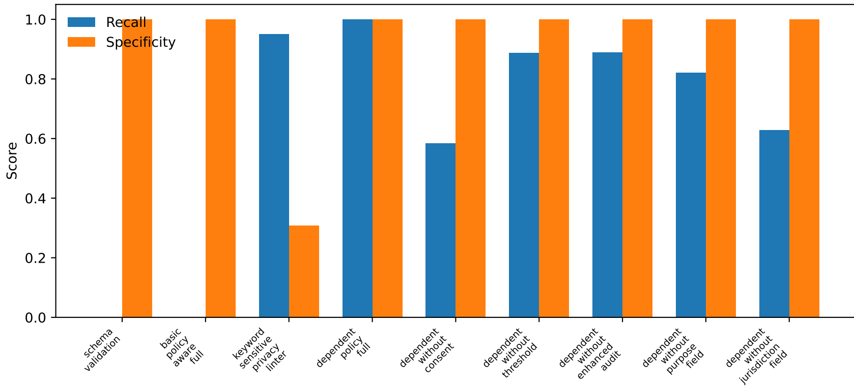
Dependent-policy detection trade-off
