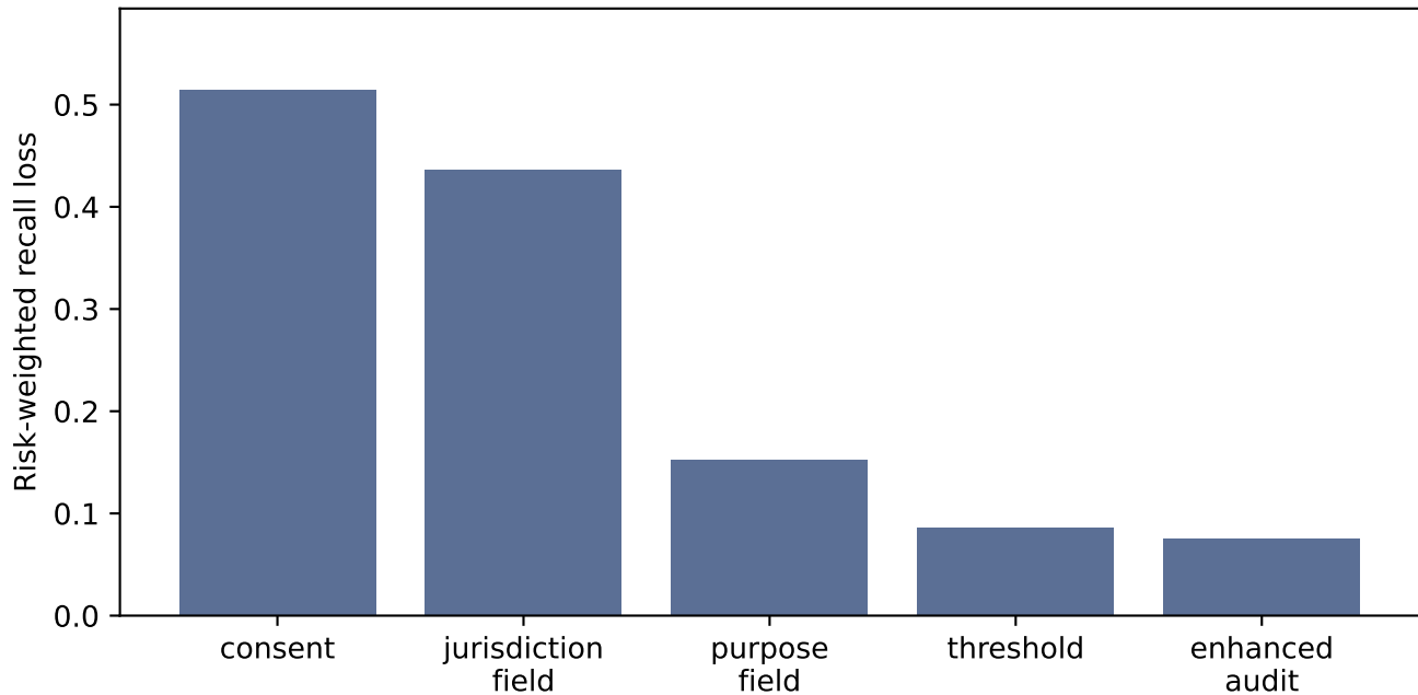
Coverage loss by removed interaction clause
