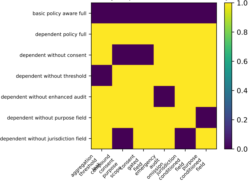
Recall by dependent violation family
