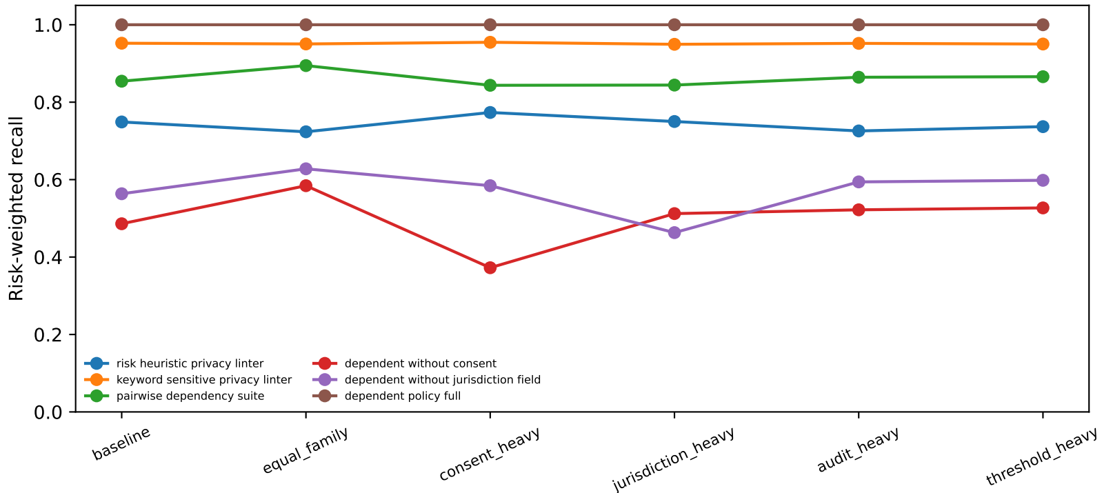
Sensitivity to severity-weight schemes
