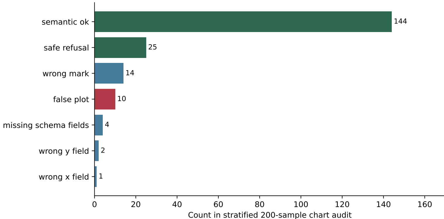
Chart-level outcomes after intent-to-Vega-Lite conversion
