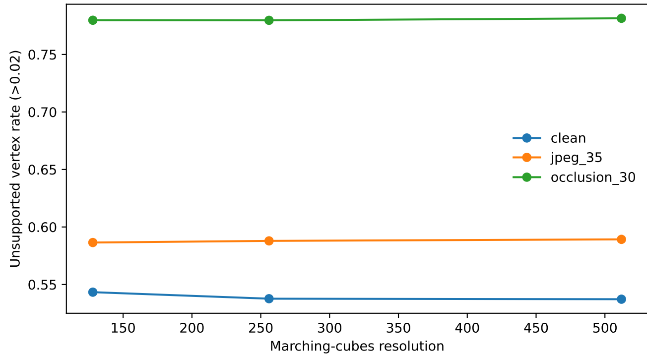
Hallucinated-surface localization
