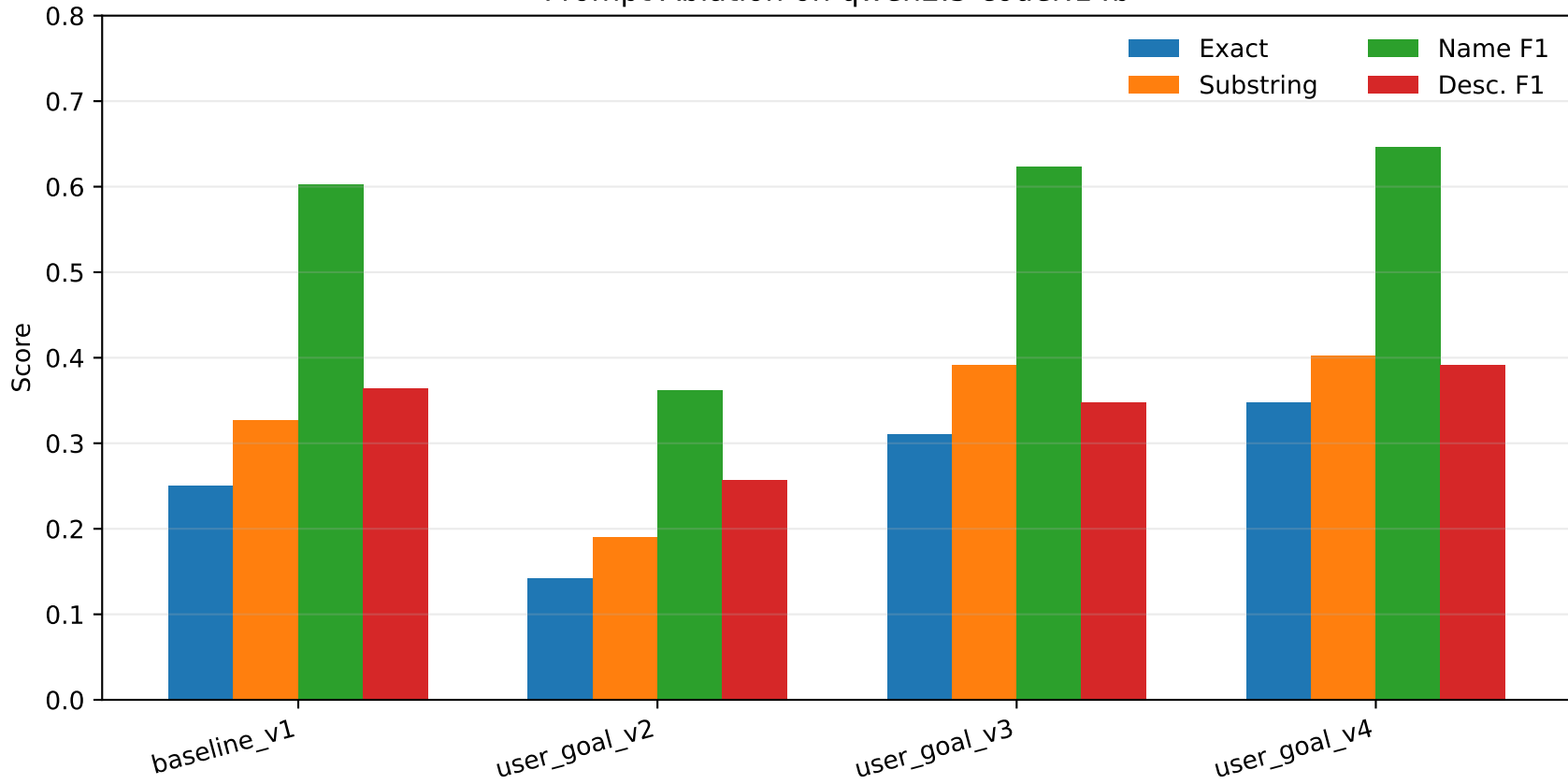
Prompt Ablation on qwen2.5-coder:14b
