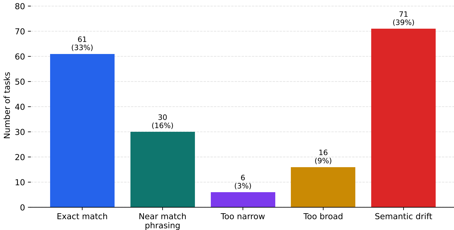
Heuristic Error Profile
