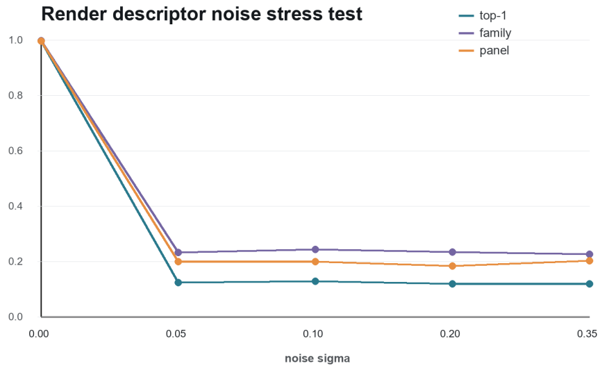
Fig. 13 Render-descriptor noise stress test on the original stratified split. The sharp drop from the clean descriptor to the perturbed descriptor shows that the high render-retrieval score depends on stable controlled-view appearance.
