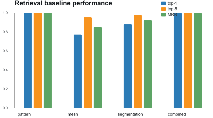
Fig. 8 Nearest-neighbor retrieval baseline performance. Mesh and segmentation features provide nontrivial category-retrieval baselines, while combined structured features nearly recover the pattern category and panel/stitch structure.
