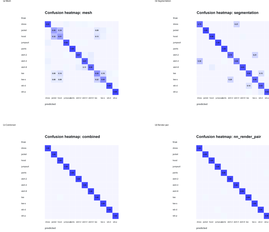
Fig. 15 Row-normalized confusion matrices for four retrieval settings: (a) mesh-only, (b) segmentation-only, (c) combined pattern, mesh, and segmentation, and (d) paired front/back render descriptors.
