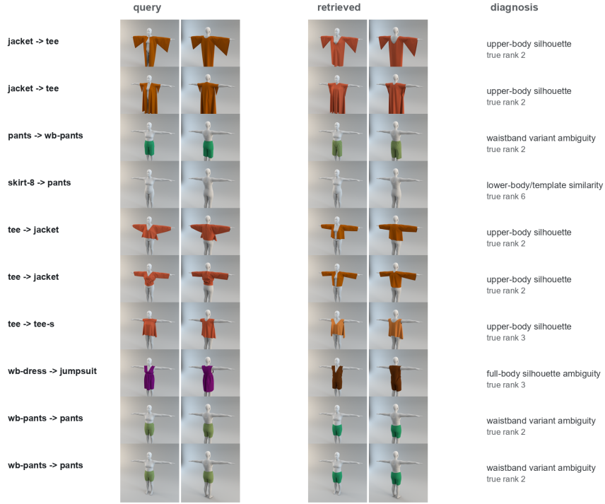
Fig. 11 All top-1 errors made by the paired render-image retrieval baseline. The errors concentrate in visually similar garment families, and the true category remains close in the nearest-neighbor ranking.
