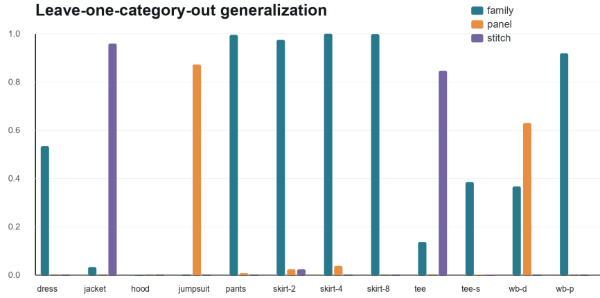
Fig. 12 Leave-one-category-out transfer for render-pair descriptors. Exact category retrieval is impossible in this protocol because the held-out category is absent from the training index; the plot therefore reports family-level, panel-exact, and stitch-exact transfer.
