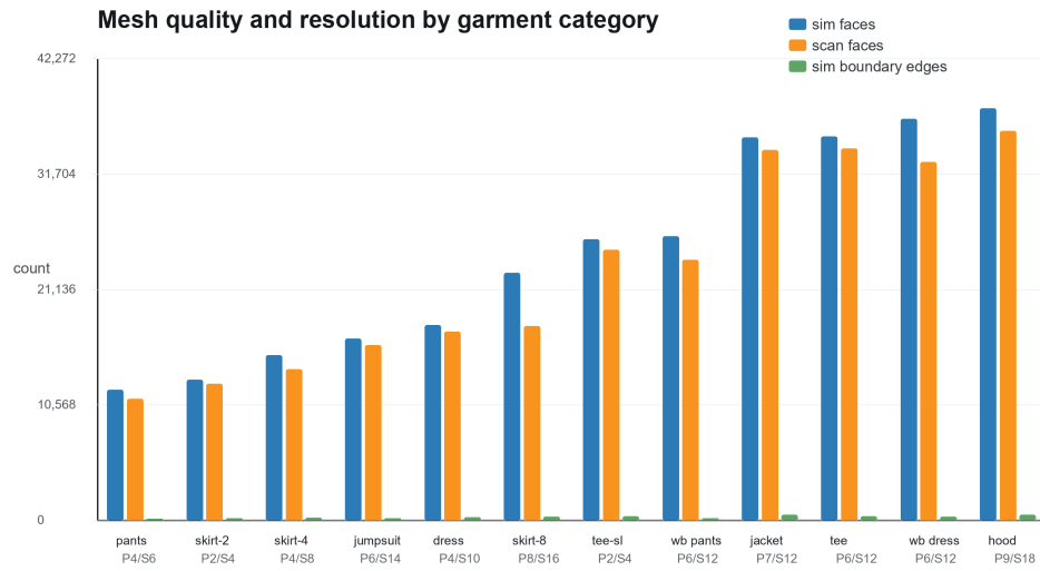
Fig. 4 Mesh-quality and resolution summary by garment category. Simulated and scan-imitation face counts provide a category-level difficulty signal; boundary edges are included as a geometric openness indicator.
